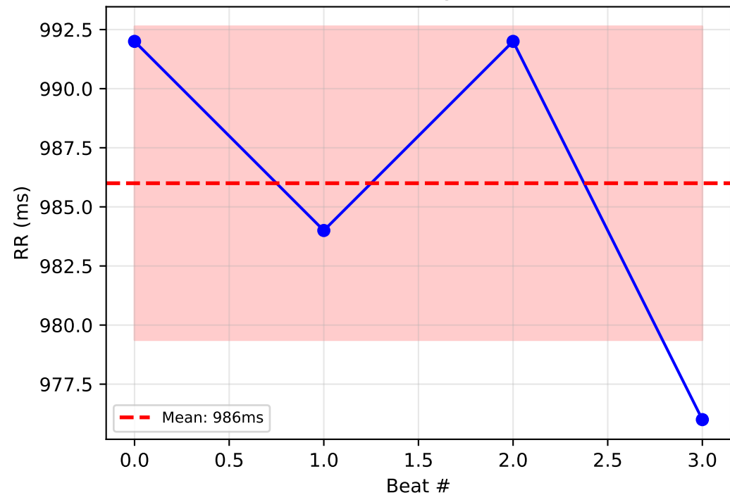
RR Tachogram
