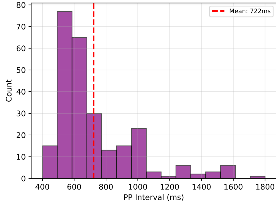
Peak-to-Peak Distribution
