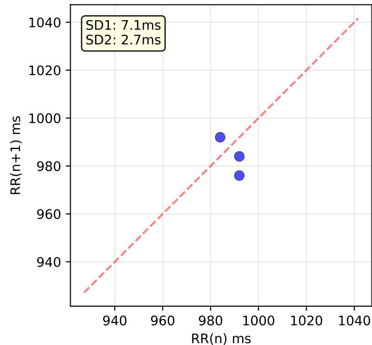
Poincaré Plot
