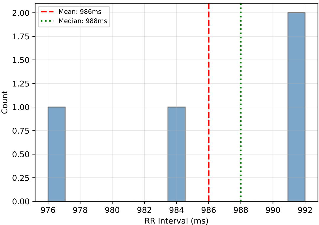
RR Distribution
