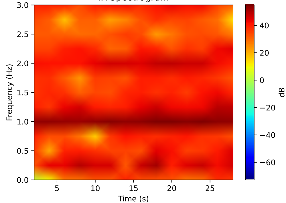
Red Spectrogram
