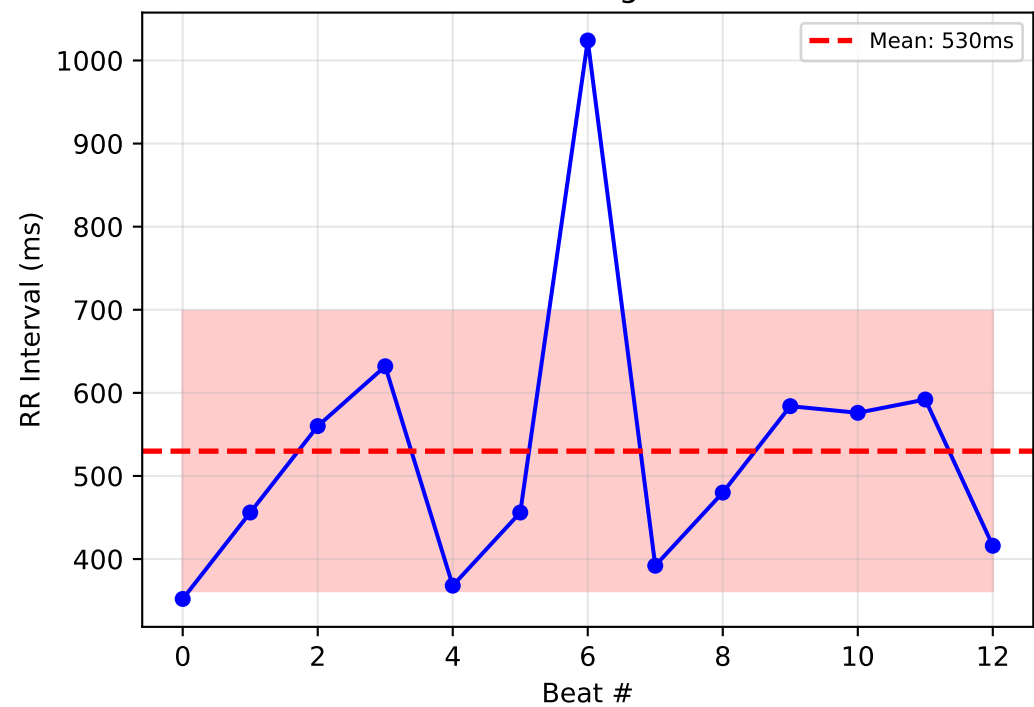
RR Tachogram
