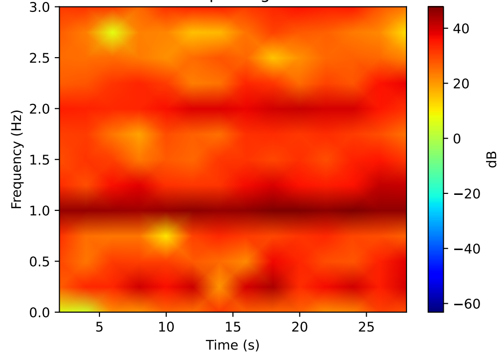
Red Spectrogram
