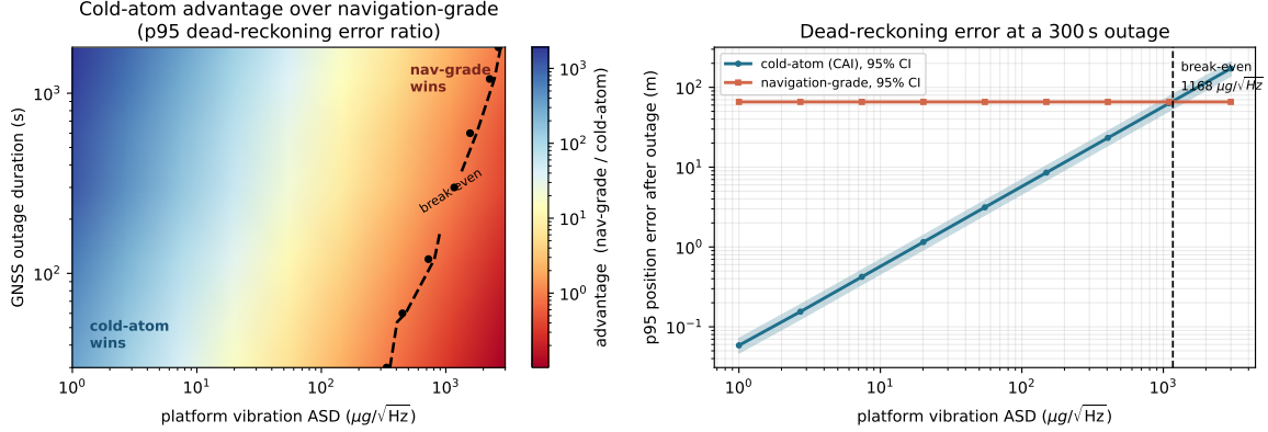
Figure 1: Inertial crossover map. Cold-atom accelerometer (Exail/Templier class, 33) versus navigation-grade strapdown (10), dead-reckoning position error (the ensemble mean of the per-run 95th percentile) as a function of outage duration and platform-vibration acceleration ASD ( \sqrt{S_a} , in \mu\text{g}/\sqrt{\text{Hz}} ). Each node is a 64-seed Monte-Carlo ensemble with a 95% bootstrap confidence interval; the dashed contour is the break-even (advantage = 1) where the navigation-grade unit matches the cold-atom sensor. The advantage is overwhelming on a quiet platform and erodes with vibration; the break-even ASD rises with outage duration. The quantum leg is a performance-model projection from laboratory-maturity device coefficients, not a measurement.
