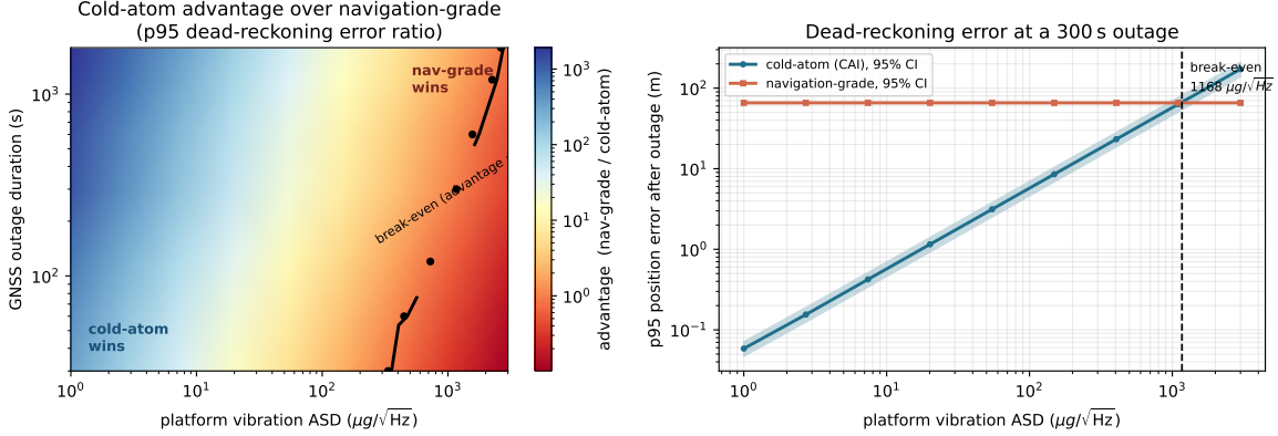
Figure 1: Inertial crossover map. Cold-atom accelerometer (Exail/Templier class, 33) versus navigation-grade strapdown (10), dead-reckoning 95th-percentile position error as a function of outage duration and platform-vibration acceleration ASD ( \sqrt{S_a} , in \mu\text{g}/\sqrt{\text{Hz}} ). Each node is a 64-seed Monte-Carlo ensemble with a 95% bootstrap confidence interval; the dashed contour is the break-even (advantage = 1) where the navigation-grade unit matches the cold-atom sensor. The advantage is overwhelming on a quiet platform and erodes with vibration; the break-even ASD rises with outage duration. The quantum leg is a performance-model projection from laboratory-maturity device coefficients, not a measurement.
