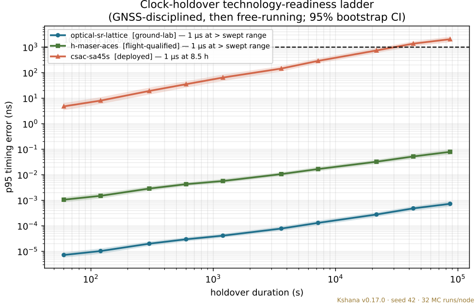
Figure 2: Clock holdover ladder. 95th-percentile timing error against a 1 \mu s budget as a function of holdover duration, for a ground-laboratory strontium optical-lattice clock (27), a flight-qualified ACES/PHARAO-class hydrogen maser, and a deployed chip-scale atomic clock. Each point is a 32-seed ensemble with a 95% bootstrap interval and carries an inline technology-readiness tag. There is no winner-flip: the optical clock dominates stability, but its margin is a laboratory figure while the maser is the realistically flown option. The CSAC reaches the budget at \approx 8.5 h.
