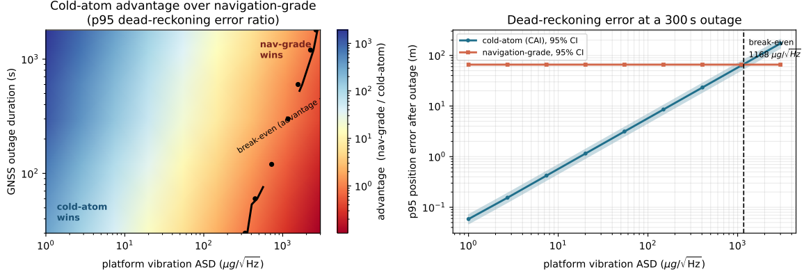
Figure 1: Inertial crossover map. Cold-atom accelerometer (Exail/Templier class, 33) versus navigation-grade strapdown (10), dead-reckoning 95th-percentile position error as a function of outage duration and platform-vibration acceleration ASD ( \sqrt{S_a} , in \mu\text{g}/\sqrt{\text{Hz}} ). Each node is a 64-seed Monte-Carlo ensemble with a 95% bootstrap confidence interval; the dashed contour is the break-even (advantage = 1) where the navigation-grade unit matches the cold-atom sensor. The advantage is overwhelming on a quiet platform and erodes with vibration; the break-even ASD rises with outage duration. The quantum leg is a performance-model projection from laboratory-maturity device coefficients, not a measurement.
