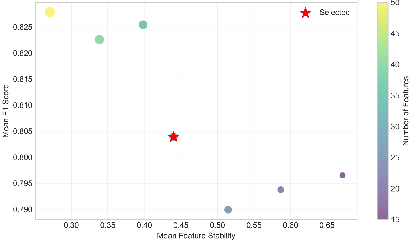
Stability vs Performance Trade-off
