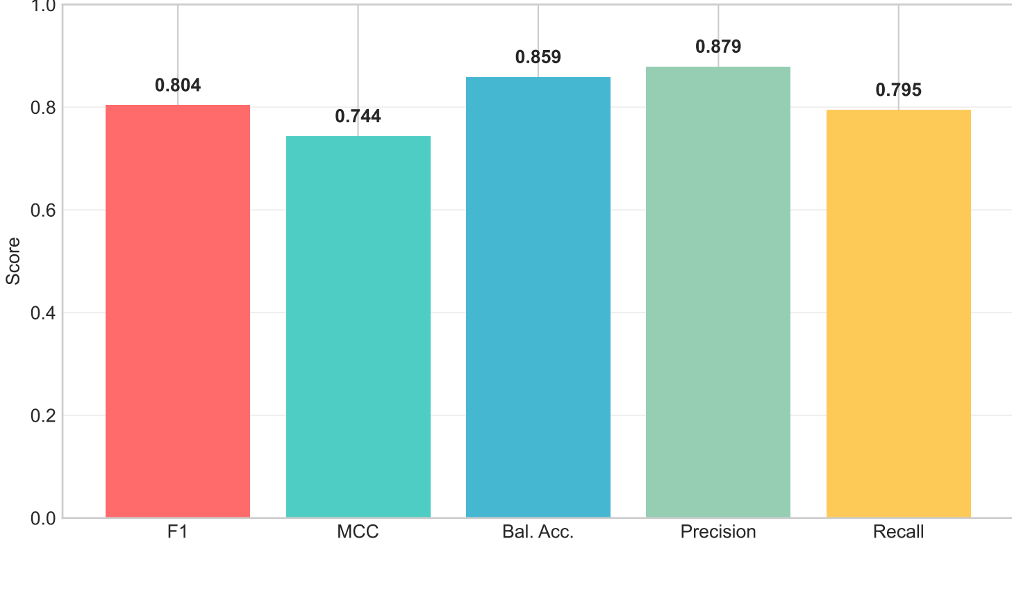
Final Model Performance Metrics
