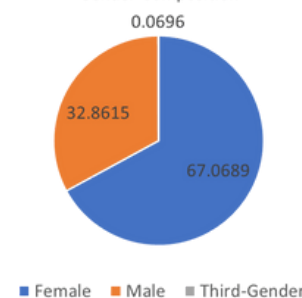
Gender Composition
