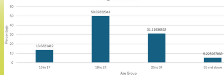
Age Distribution
