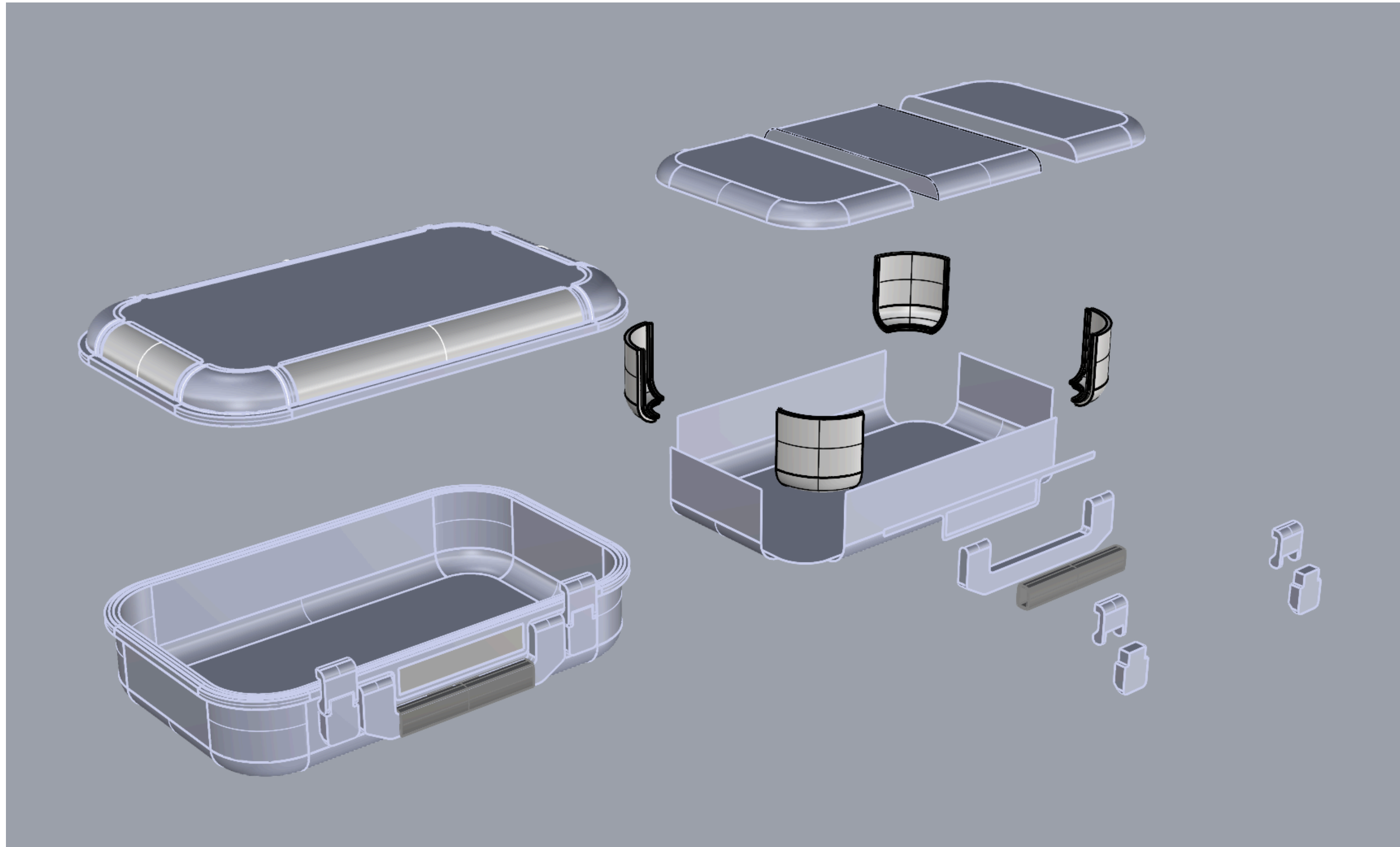
Assembly Diagram (Foamboard, PLA, and Cast Acrylic)
