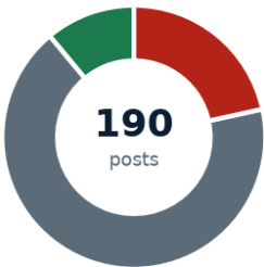
Sentiment mix
