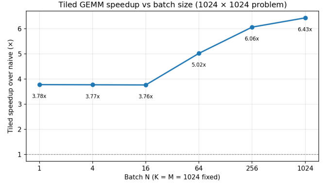
Fig. 4. Tiled-GEMM speedup over the naive kernel as the batch dimension N sweeps from 1 to 1024 at a fixed 1024 \times 1024 weight shape. The plateau at \sim 3.8 \times for N \leq 16 reflects the regime in which the output M -tile is fully populated but only one K -panel is reused; the further climb to 6.43 \times at N=1024 reflects full reuse along all three dimensions.
