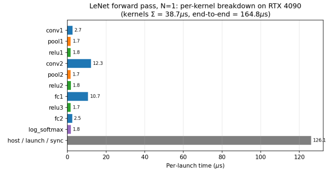
Fig. 6. Per-kernel contribution to the N=1 LeNet forward pass. The ten CUDA kernels together account for \sim 39\mu s ; the remaining \sim 126\mu s (the bottom bar) is host-side launch submission, CUDA runtime overhead, and synchronization on the final device-to-host copy. Conv2 and fc1 dominate actual kernel work; every other kernel is within noise of the \sim 1.7\mu s launch floor for a trivial CUDA kernel on this platform.
