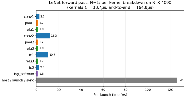
Fig. 3. Per-kernel contribution to the N=1 LeNet forward pass. The ten CUDA kernels together account for \sim 39 \mu s ; the remaining \sim 126 \mu s (the bottom bar) is host-side launch submission, CUDA runtime overhead, and synchronization on the final device-to-host copy. Conv2 and fc1 dominate actual kernel work; every other kernel is within noise of the \sim 1.7 \mu s launch floor for a trivial CUDA kernel on this platform.
