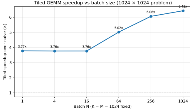
Fig. 2. Tiled-GEMM speedup over the naive kernel as the batch dimension N sweeps from 1 to 1024 at a fixed 1024 \times 1024 weight shape. The plateau at \sim 3.8\times for N \leq 16 reflects the regime in which the output M -tile is fully populated but only one K -panel is reused; the further climb to 6.43\times at N=1024 reflects full reuse along all three dimensions.
