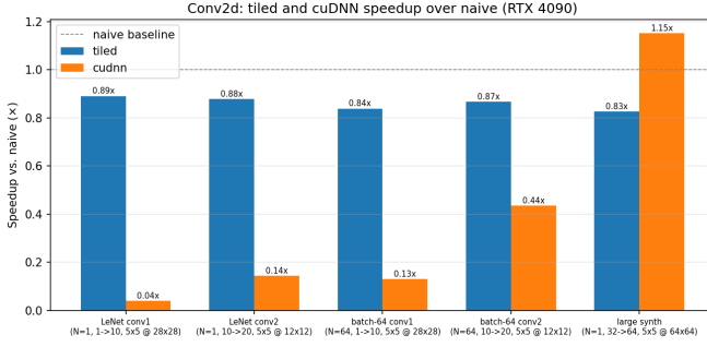
Fig. 1. Convolution speedup over the naive direct kernel on RTX 4090. cuDNN (IMPLICIT_PRECOMP_GEMM with FMA math to match FP32 numerics) pays a fixed per-launch overhead that dominates at LeNet scale and only crosses over on the larger 32→64 synthetic shape.
