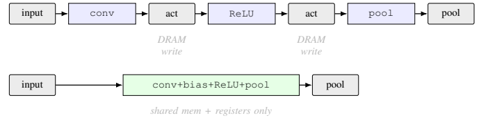
Fig. 7. Memory-traffic view of the fused stage. Top: three separate kernels, with the full post-conv and post-ReLU activations written to and read from DRAM between launches. Bottom: one kernel, with intermediate values kept in shared memory and registers; only the pool output hits DRAM.
