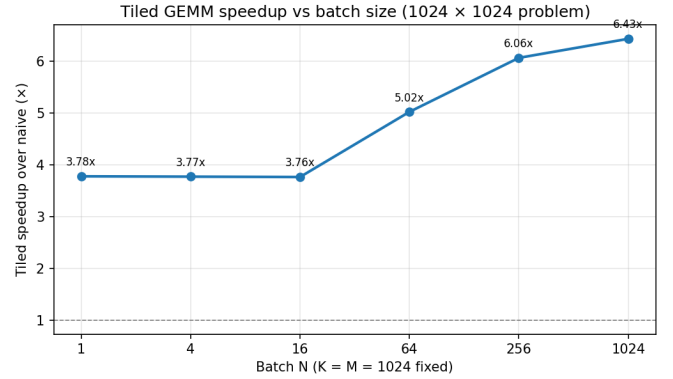
Fig. 4. Tiled-GEMM speedup over the naive kernel as the batch dimension N sweeps from 1 to 1024 at a fixed 1024 \times 1024 weight shape. The plateau at \sim 3.8 \times for N \leq 16 reflects the regime in which the output M -tile is fully populated but only one K -panel is reused; the further climb to 6.43 \times at N=1024 reflects full reuse along all three dimensions.
