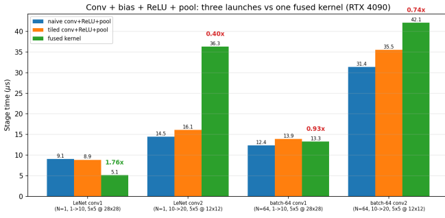
Fig. 8. Conv+bias+ReLU+pool stage time ( \mu s) on RTX 4090 across four shapes. Bars compare the three-kernel baseline (conv_naive \rightarrow ReLU \rightarrow max_pool2d, and the same with tiled conv) against the single fused kernel. Speedup over the naive three-kernel sequence is printed above the fused bar (green where the fused kernel wins, red where it loses).
