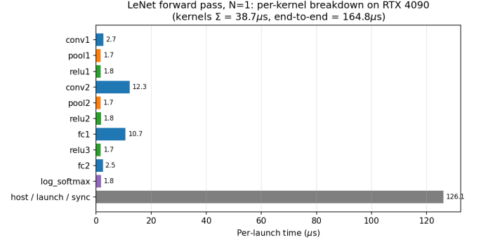
Fig. 6. Per-kernel contribution to the N=1 LeNet forward pass. The ten CUDA kernels together account for \sim 39\ \mu\text{s} ; the remaining \sim 126\ \mu\text{s} (the bottom bar) is host-side launch submission, CUDA runtime overhead, and synchronization on the final device-to-host copy. Conv2 and fc1 dominate actual kernel work; every other kernel is within noise of the \sim 1.7\ \mu\text{s} launch floor for a trivial CUDA kernel on this platform.
