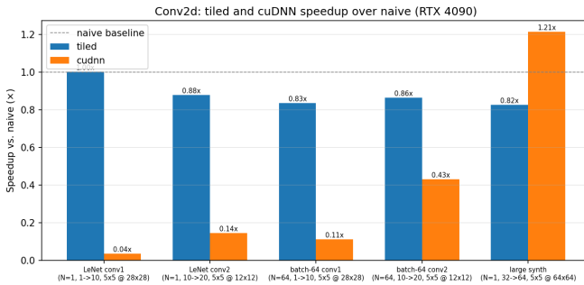
Fig. 2. Convolution speedup over the naive direct kernel on RTX 4090. cuDNN (IMPLICIT_PRECOMP_GEMM with FMA math to match FP32 numerics) pays a fixed per-launch overhead that dominates at LeNet scale and only crosses over on the larger 32 \rightarrow 64 synthetic shape.
