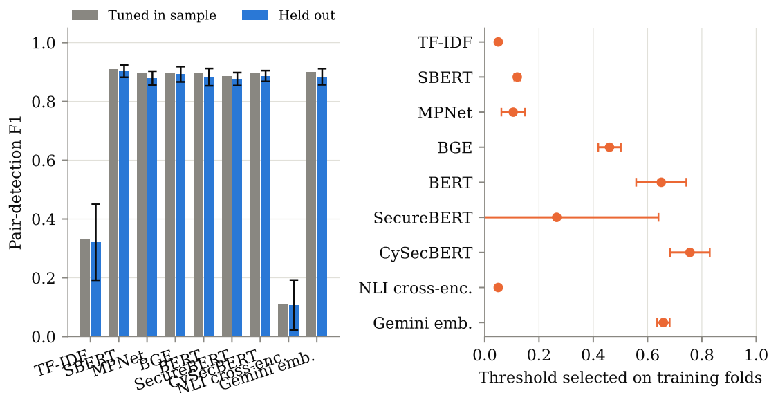
Figure 5.6: Left: pair-detection F1 with the threshold tuned on the same pairs it is scored on, against the held-out mean of 20 repeats of stratified 5-fold cross-validation (error bars, one standard deviation). Right: the threshold each set of training folds selected.
