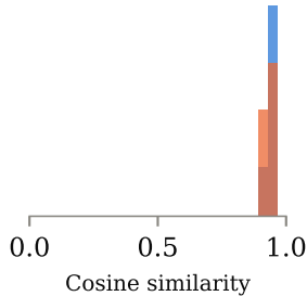
SecureBERT
