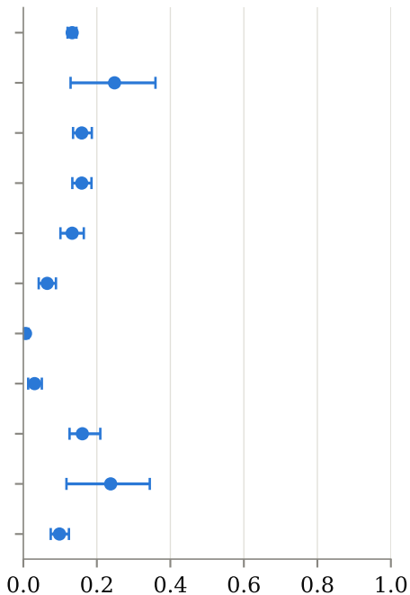
Classification macro-F1
