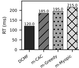
(c) Response time
