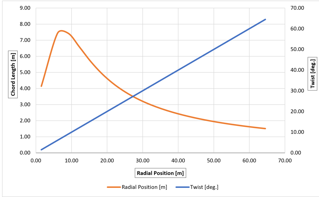
Figure 1: Analytical spanwise chord distribution and smoothed structural twist angle ( \theta_{\text{twist}} ) derived via Schmitz's optimization theory across 21 blade stations.
