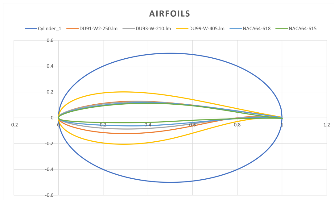
Figure 2: Normalized geometric profiles showing thickness distributions across the allocated airfoil families
