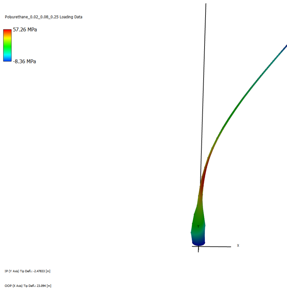
Figure 9: Aeroelastic static tip deflection and stress distribution visualization for the Polyurethane elastomeric configuration under rated structural loading conditions
