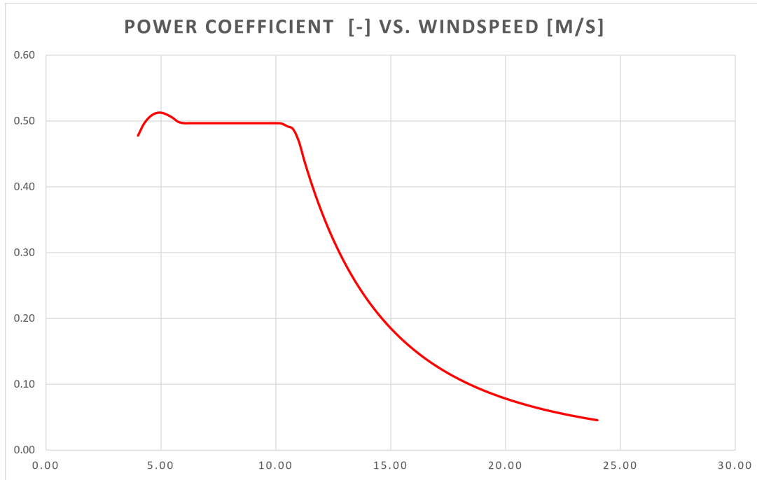
Figure 7: 3D rotor aerodynamic power coefficient ( C_p ) across the operational velocity envelope, simulated utilizing the DTU Polynomial Blade Element Momentum (Poly BEM) solver.
