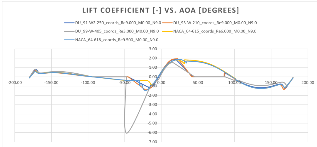
Figure 4: Viscous section lift coefficients ( C_L ) as a function of angle of attack up to the localized XFOIL panel solver numerical convergence limits
