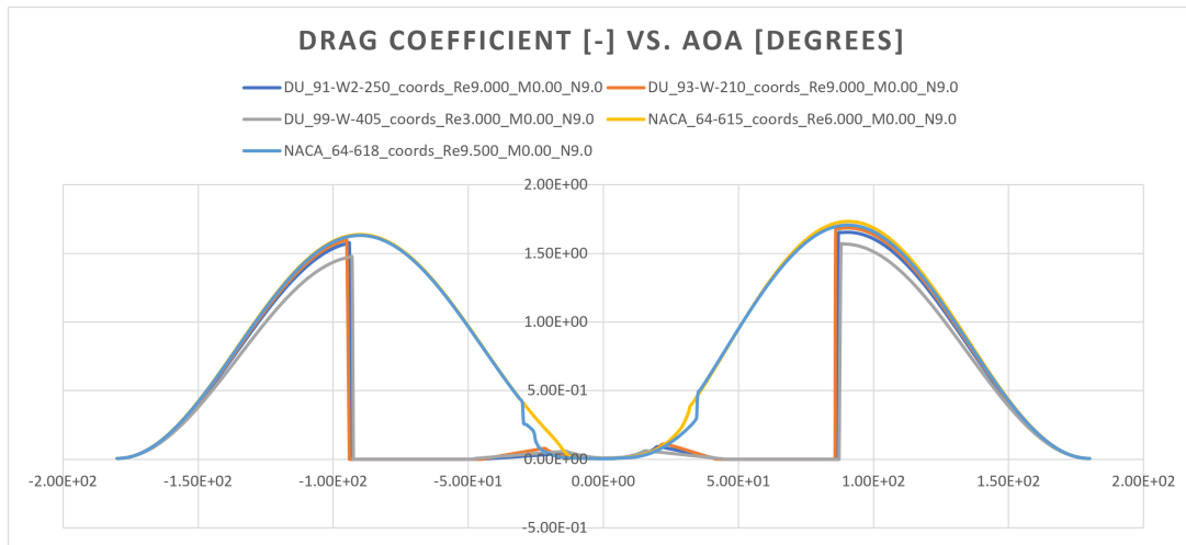
Figure 5: Profile drag coefficients ( C_D ) highlighting the drag penalty divergence between blunt structural root sections and slender aerodynamic tip sections
