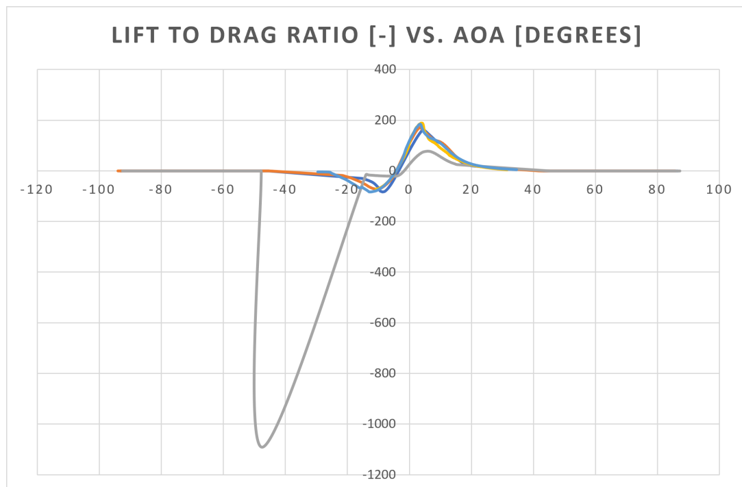
Figure 3: Two-dimensional aerodynamic lift-to-drag efficiency curves ( \varepsilon = C_L/C_D ) across operational angles of attack for specific section Reynolds numbers ( Re = 3.0 \times 10^6 to 9.5 \times 10^6 )
