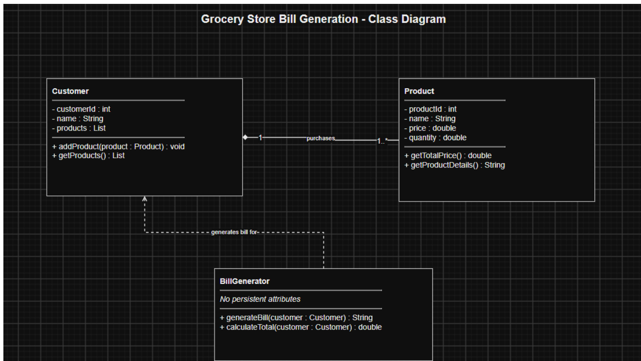
Figure 4: Grocery Store Bill Generation – Class Diagram
