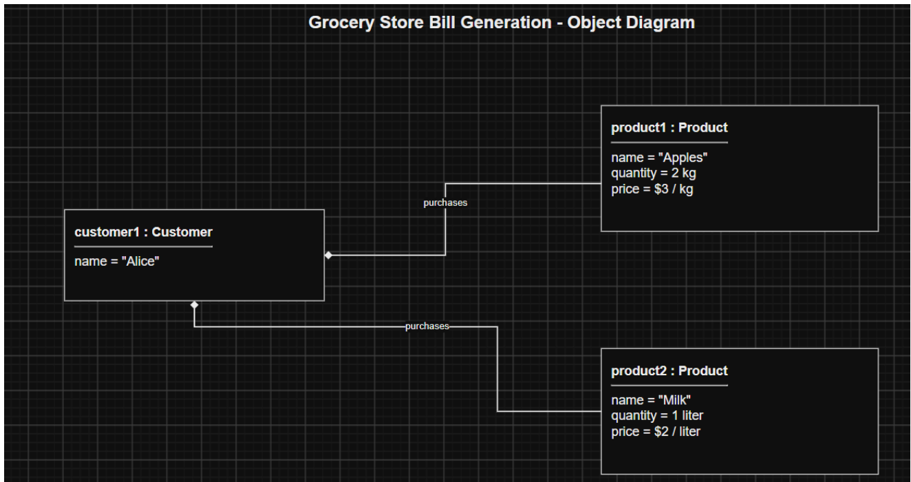
Figure 5: Grocery Store Bill Generation – Object Diagram
