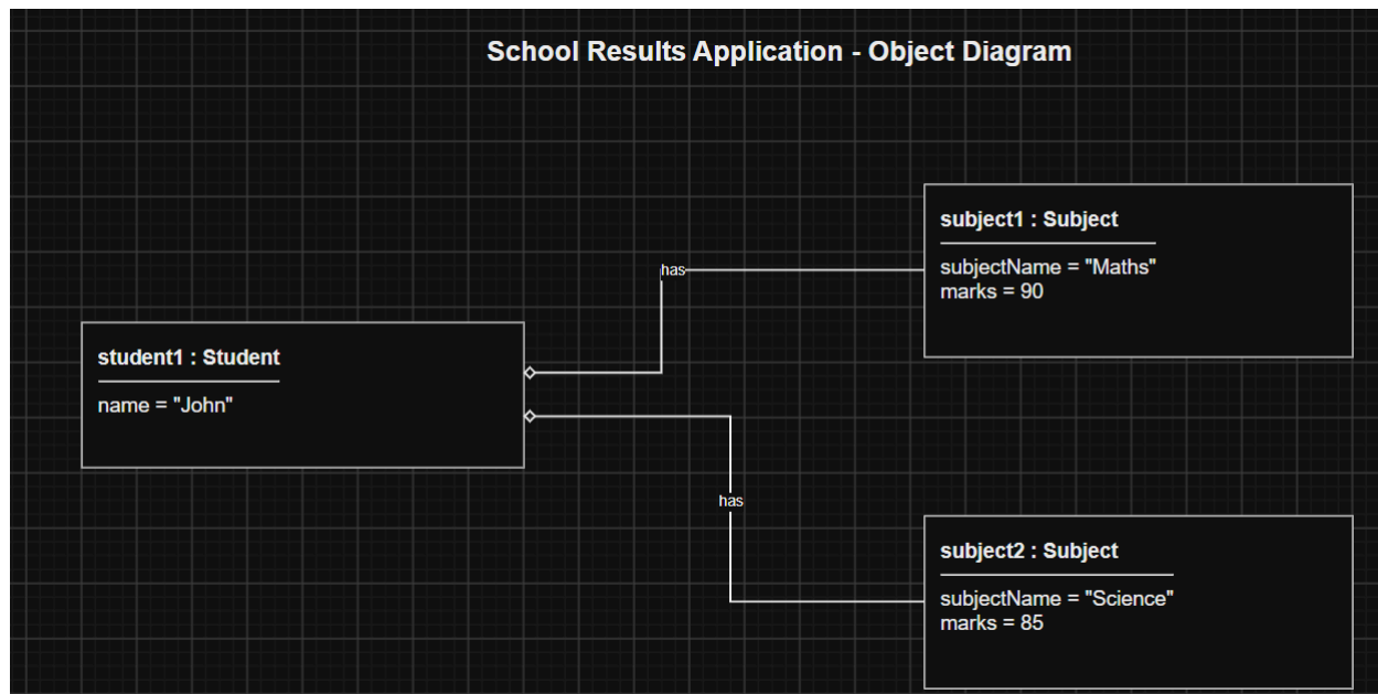
Figure 2: School Results Application – Object Diagram
