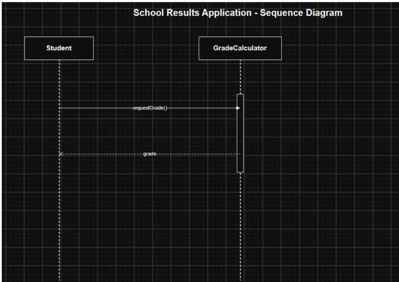
Figure 3: School Results Application – Sequence Diagram
