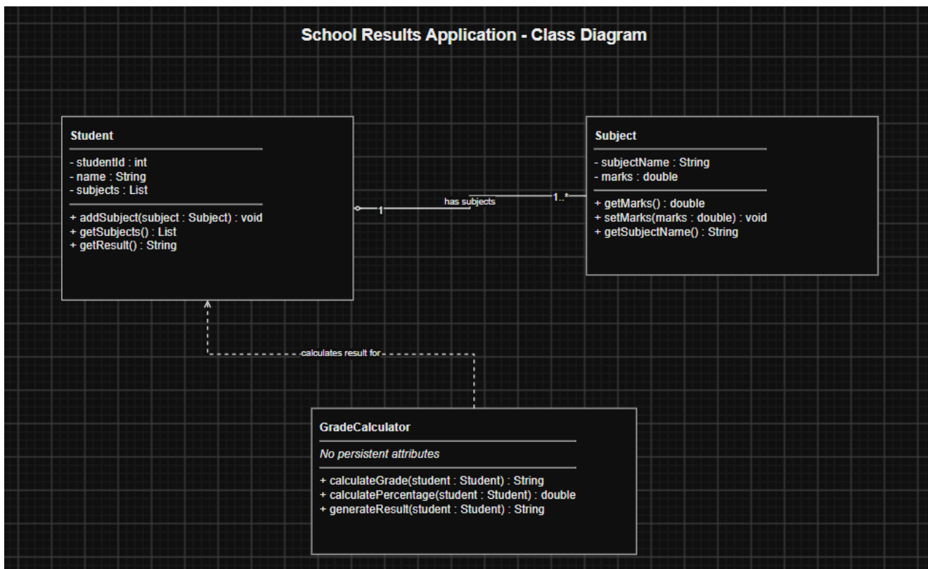
Figure 1: School Results Application – Class Diagram
