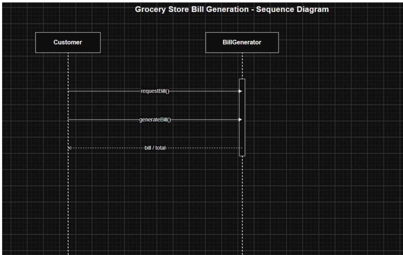
Figure 6: Grocery Store Bill Generation – Sequence Diagram
