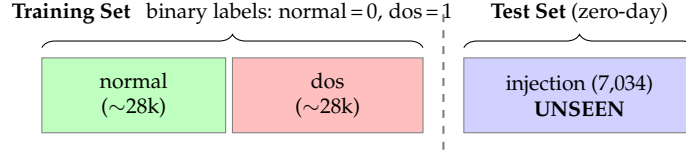
Figure 3: Zero-day experimental split. The model trains on normal and DoS traffic only (binary classification), then is tested on injection attacks — an entirely unseen class. High detection rate indicates genuine generalization beyond memorized attack patterns.
