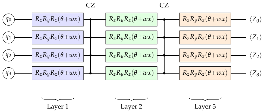
Figure 8: Multi-qubit data re-uploading circuit (4 qubits, 3 layers). Each qubit independently applies parameterized R_z R_y R_z rotations that mix input data x with trainable weights, with nearest-neighbor CZ gates entangling the qubits between layers. The final output is the average of the per-qubit \langle Z \rangle measurements, expressed as a single Hamiltonian measurement \langle H \rangle = \frac{1}{n} \sum_q Z_q . Total: 6 \times 4 \times 3 = 72 parameters per binary classifier.
