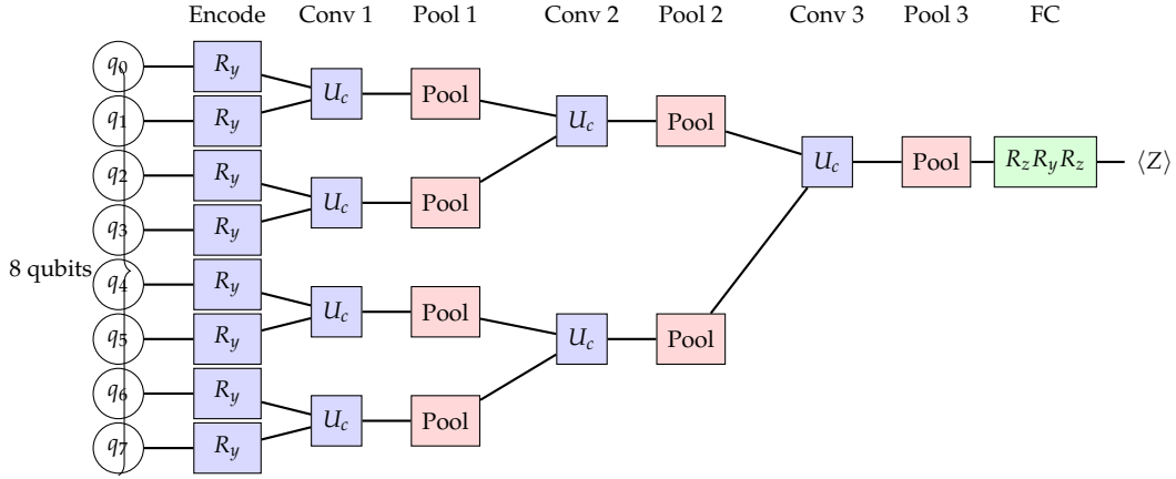
Figure 6: QCNN architecture ( 8 \rightarrow 4 \rightarrow 2 \rightarrow 1 qubits). Input features are encoded via R_y rotations. Three convolutional-pooling stages hierarchically reduce the circuit width. Each convolutional unitary U_c applies 6 parameterized rotations; each pooling layer uses CRZ–CRY (2 parameters) to transfer information before discarding one qubit. A final R_z R_y R_z layer on the remaining qubit produces the output \langle Z \rangle \in [-1, +1] . Total: 27 parameters per binary classifier.
