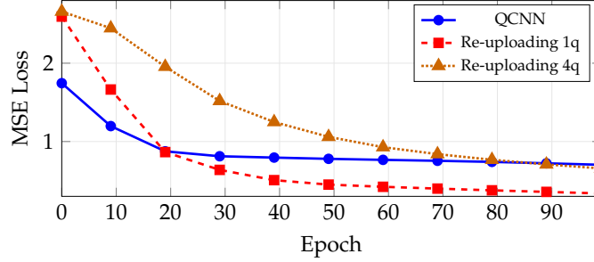
Figure 4: Training loss curves for quantum models on the standard 3-class setting (100 epochs, 500 training samples, seed 0). All three models converge, with the single-qubit re-uploading reaching the lowest loss (0.34).
