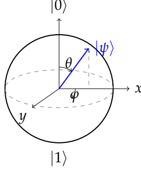
Figure 1: The Bloch sphere. Any pure single-qubit state |\psi\rangle corresponds to a point on the surface, parameterized by angles \theta and \varphi .
