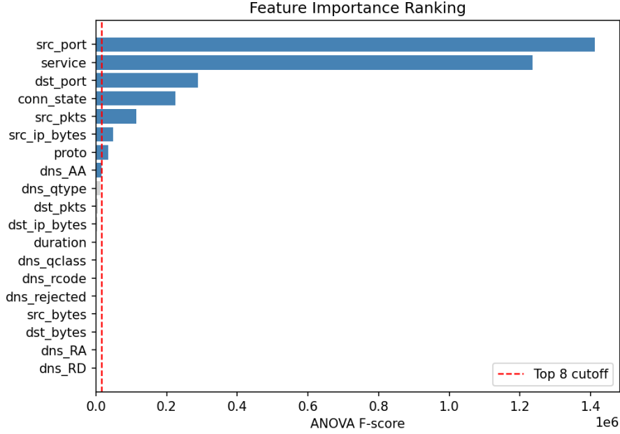
Figure 2: ANOVA F-score ranking of the 19 candidate features. The top 8 (blue) are selected for quantum encoding; the red dashed line marks the cutoff.
