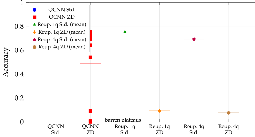
Figure 5: Accuracy distribution across 10 random initialization seeds for each quantum model and task (500 samples, 100 epochs). QCNN points are individual seeds; re-uploading is shown as a single mean marker because its per-seed values are tightly clustered (standard deviations 0.011–0.039). The QCNN zero-day task exhibits three barren-plateau collapses at \leq 9\% , while seven seeds achieve 54–76%. All other model–task combinations are stable across seeds.
