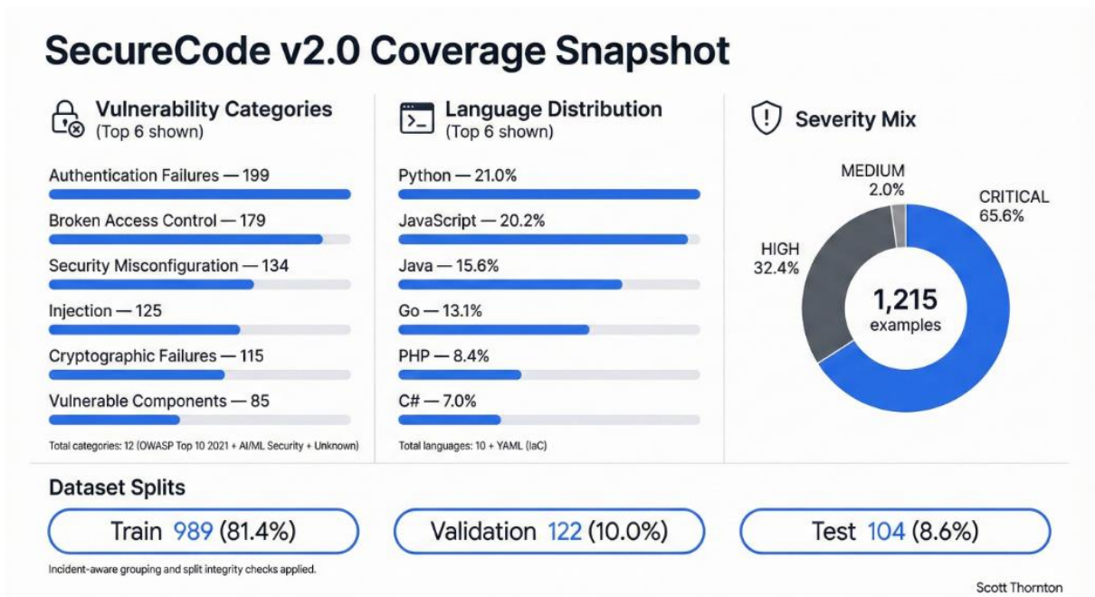
Figure 0-1.1: Secure-Code v2.0 Coverage
