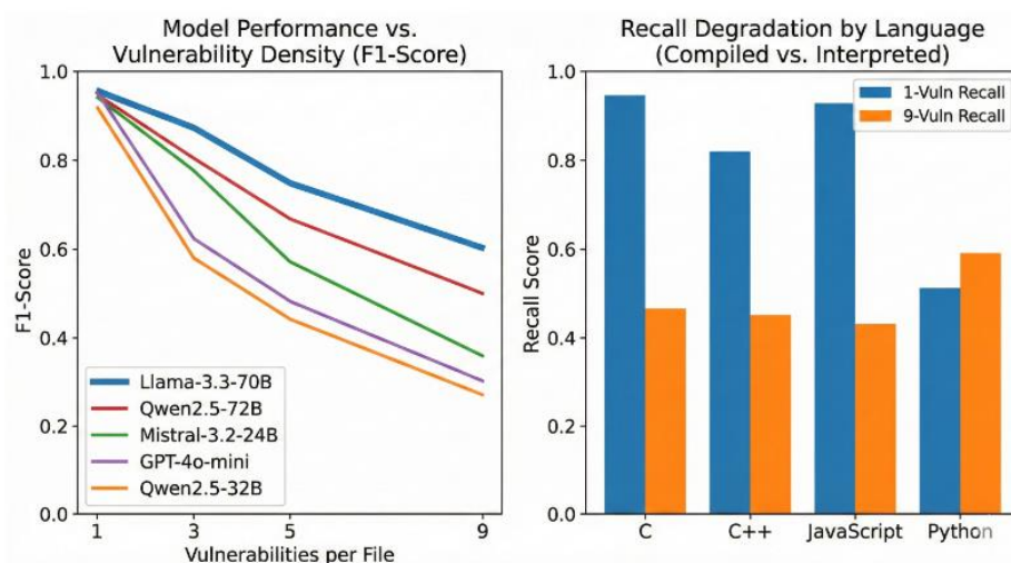
Figure 2.0-2: Evaluation of LLMs on Code Vulnerability Detection Across Varying Density and Language Types [35].
