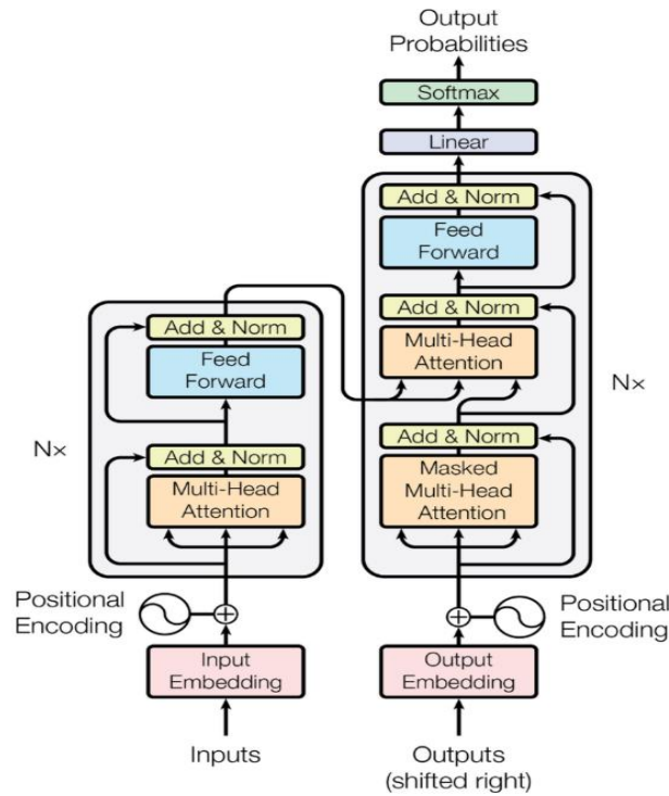
Figure 2.1: Transformer's Architecture
