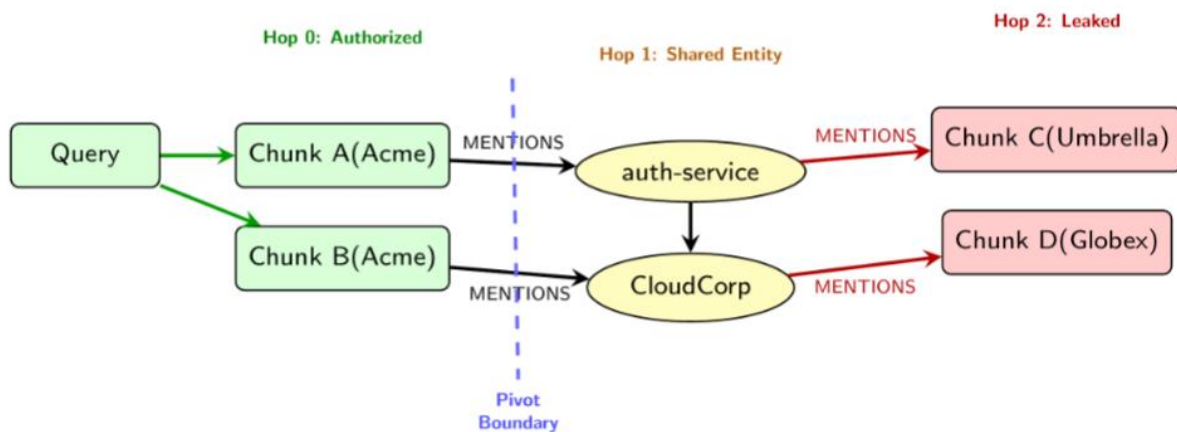
Figure 2.0-3: The retrieval pivot attack surface. Vector retrieval returns authorized seed chunks (hop 0, green). BFS expansion traverses MENTIONS edges to shared entity nodes (hop 1, yellow), then onward to unauthorized chunks from other tenants (hop, red). The pivot boundary (dashed) is where authorization must be re-checked. D1 filters at this boundary, eliminating all leakage [37].
