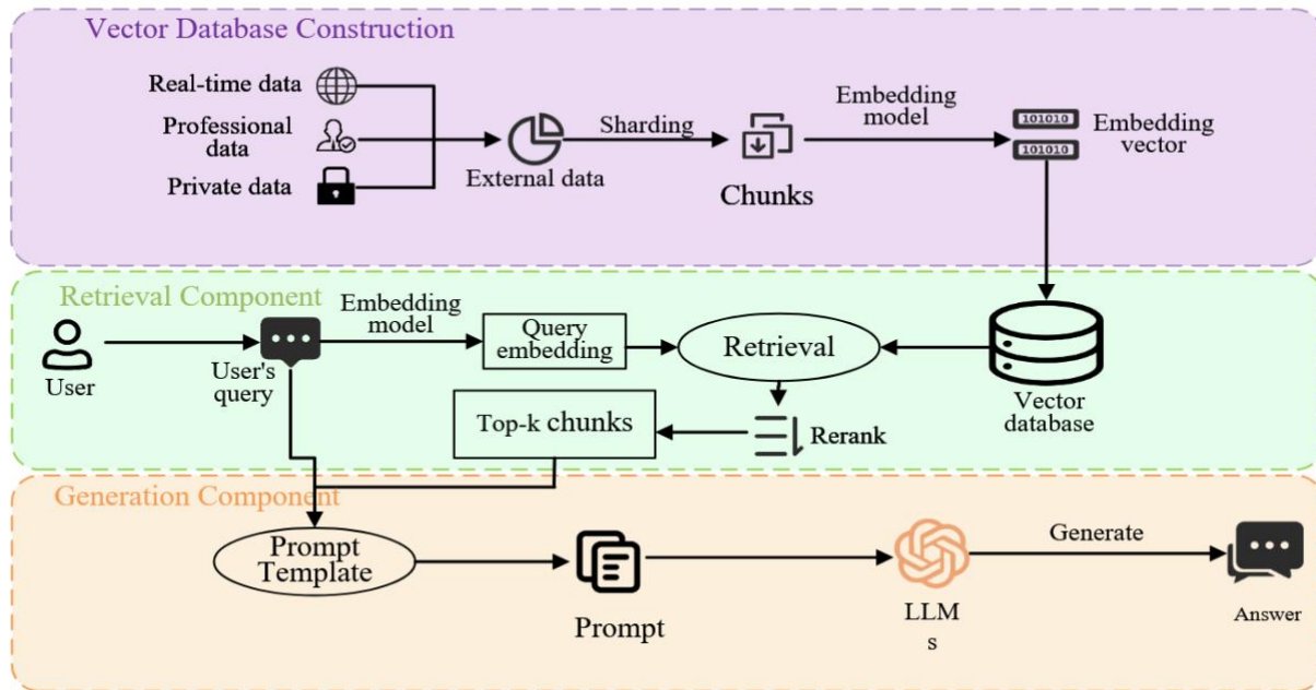
Figure 0-1.2: RAG Technical Workflow [12].
