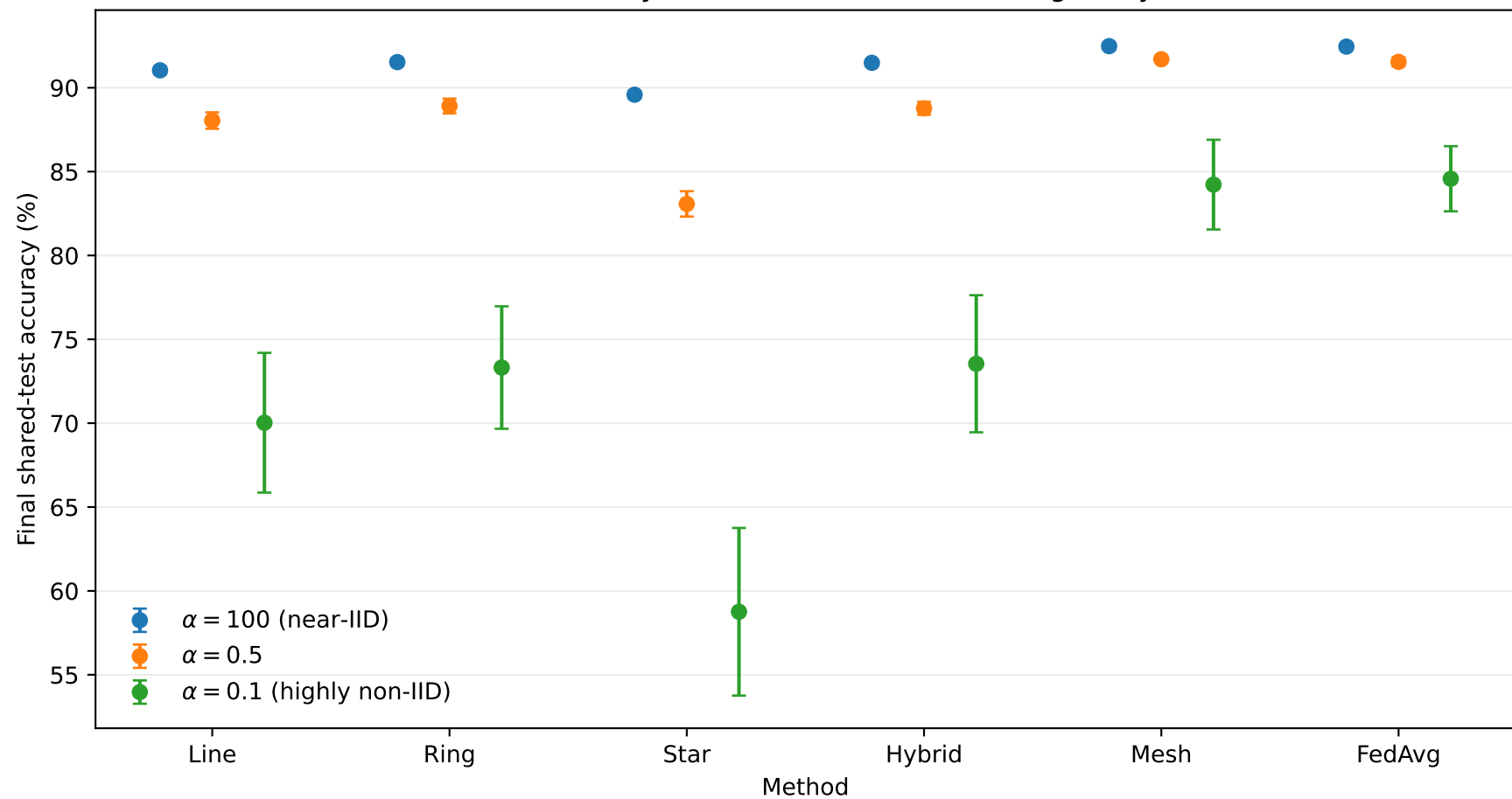
Final-round accuracy across methods and heterogeneity levels
