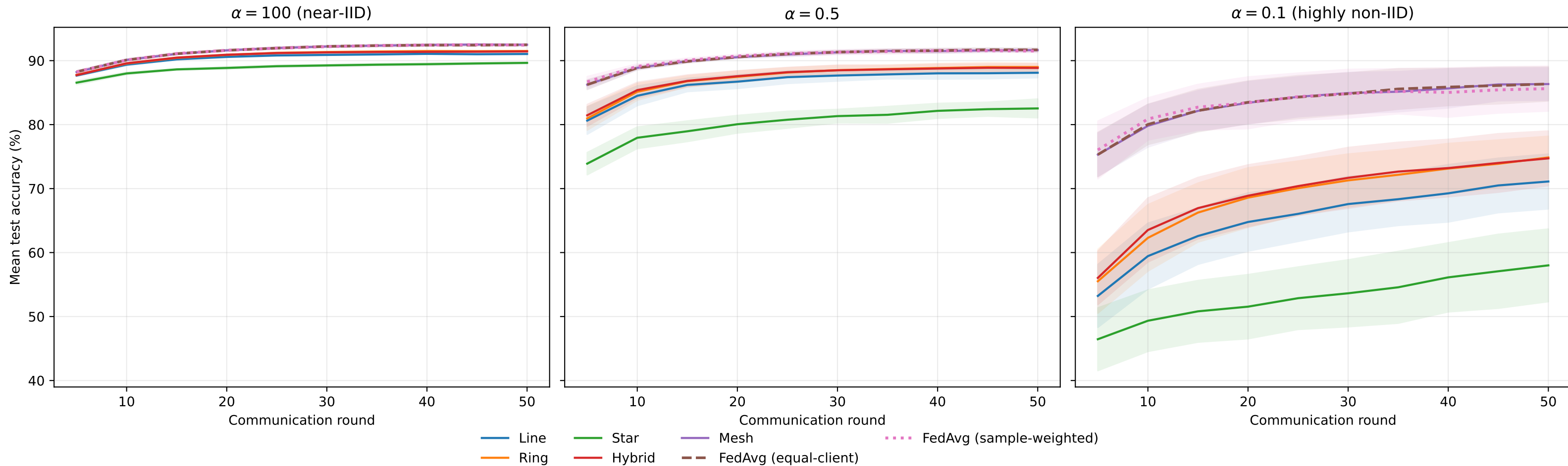
Convergence across communication topologies and FedAvg baselines
