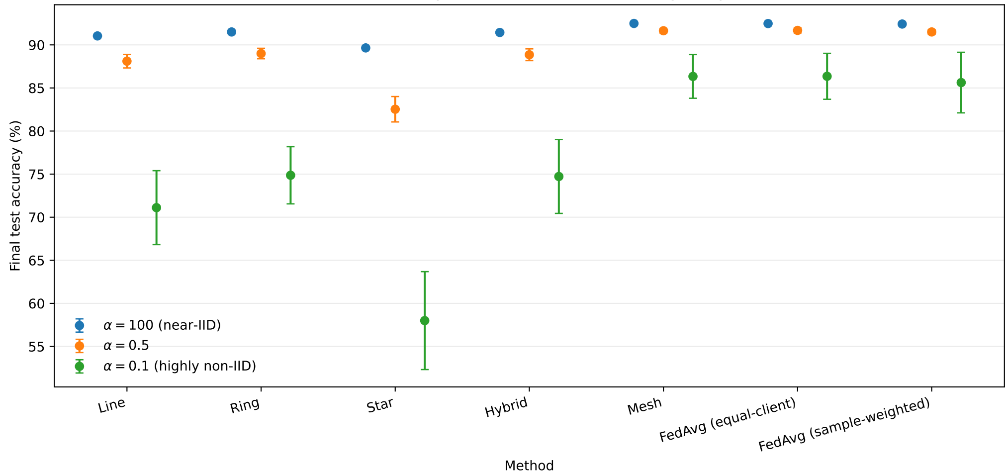
Final-round accuracy across methods and heterogeneity levels
