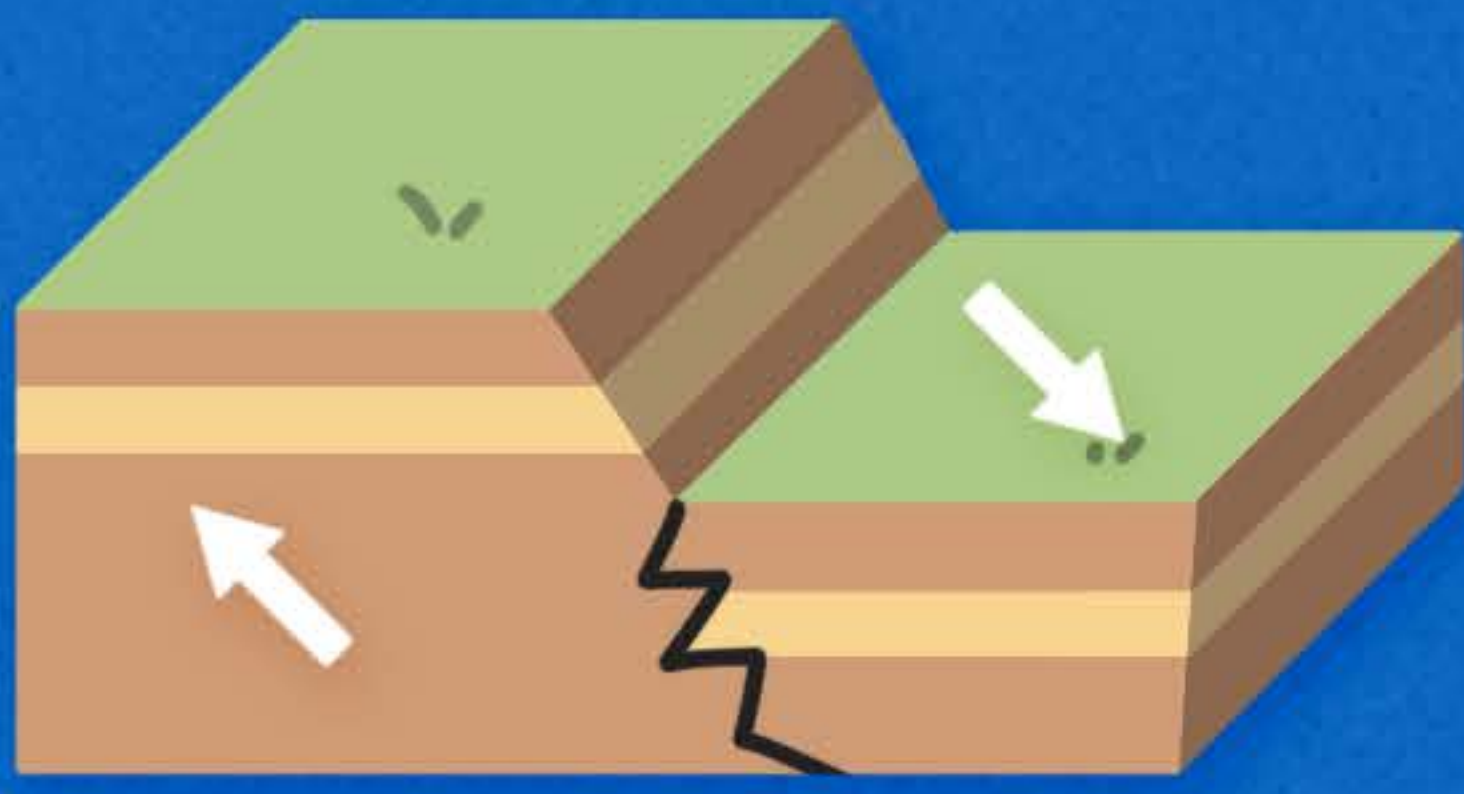
Normal
