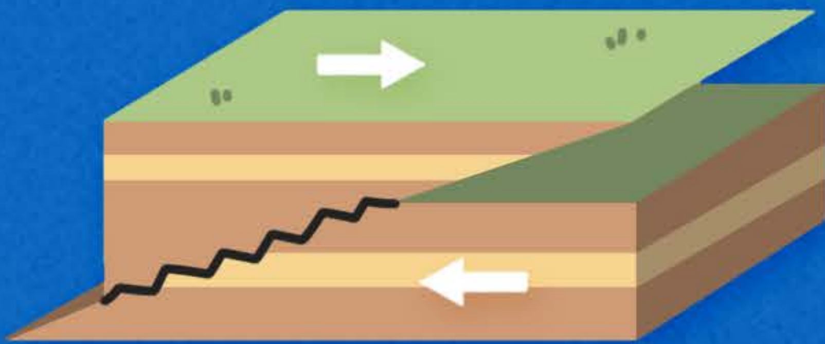
Thrust
