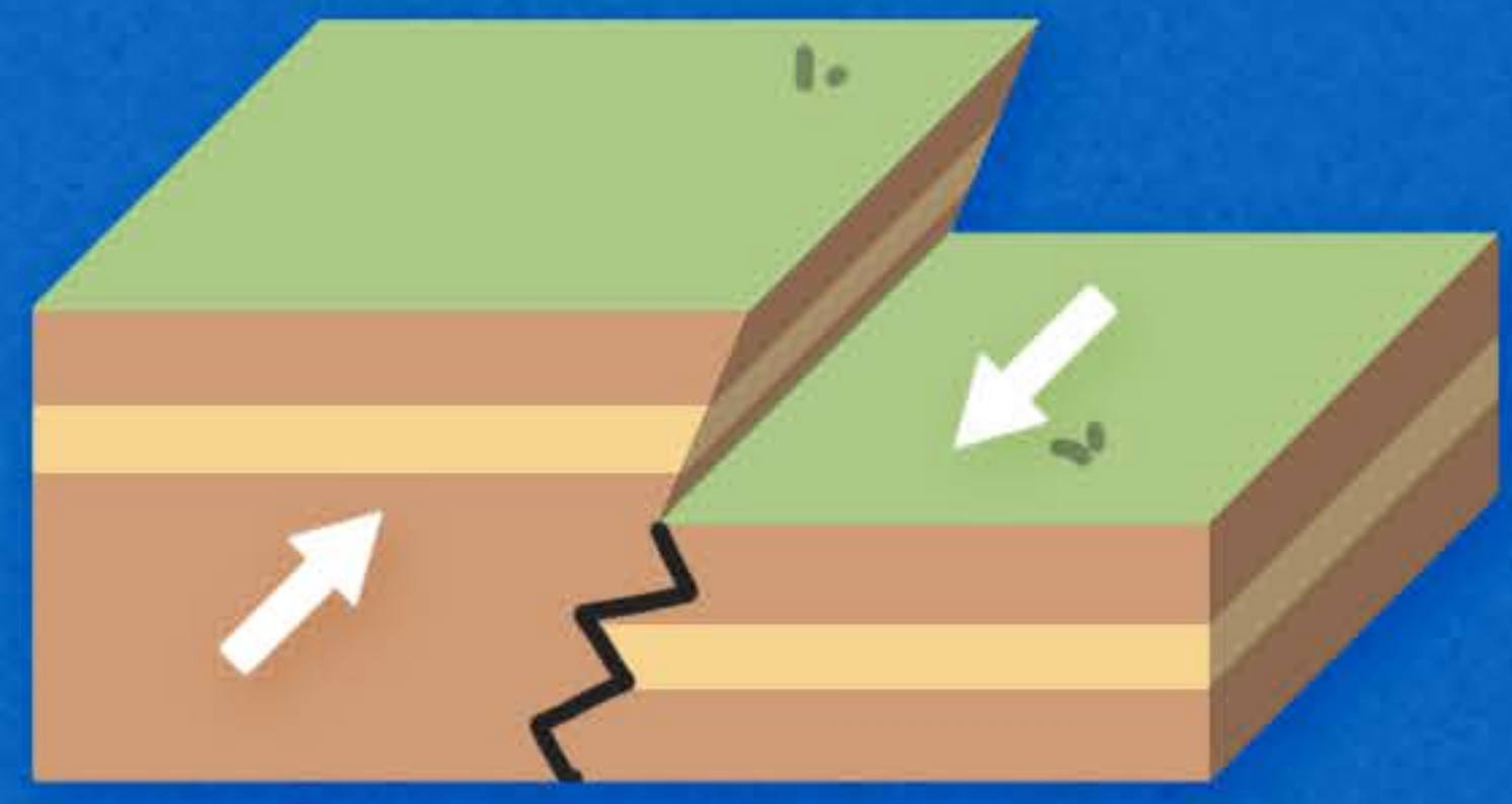
Reverse
