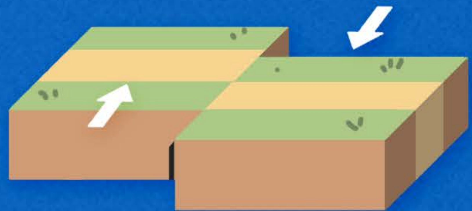
Strike-Slip
