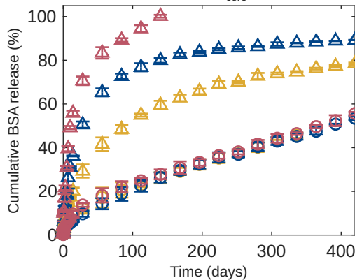
Large microcapsules ( R_{\text{core}} = 0.8225 \text{ mm} )
