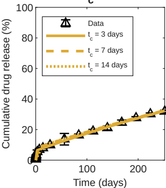
5% salt leaching (Best t_c = 3 days)
