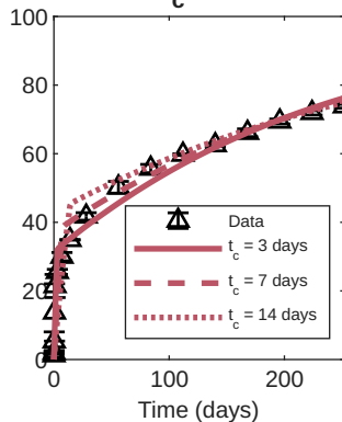
10% salt leaching (Best t_c = 3 days)
