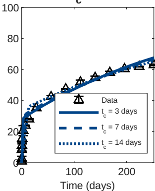
7.5% salt leaching (Best t_c = 3 days)
