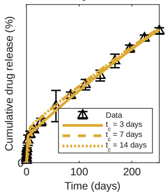
5% salt leaching (Best t_c = 3 days)
