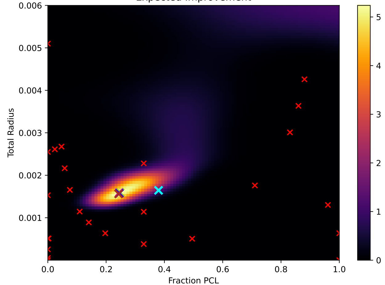
Expected Improvement
