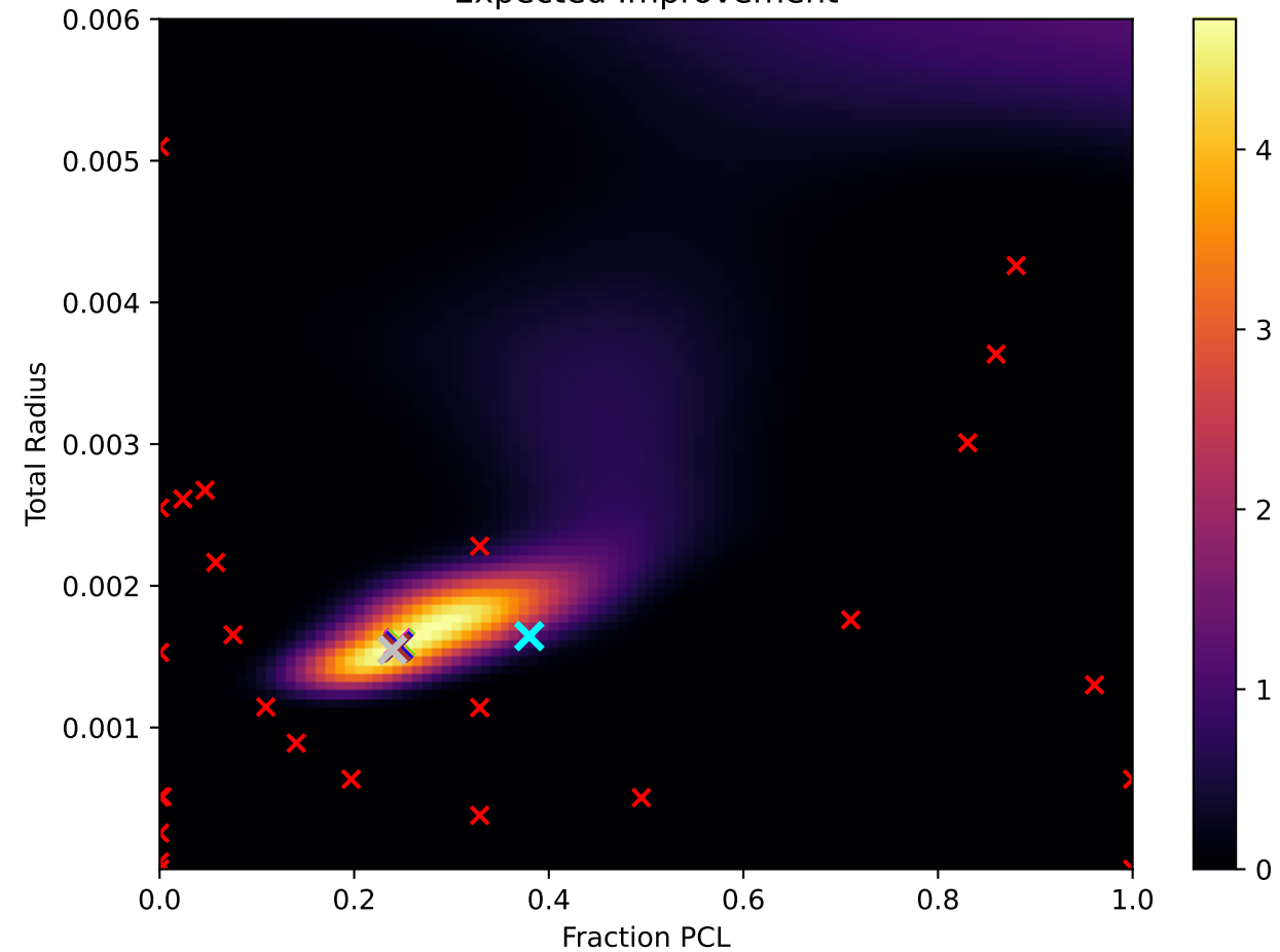
Expected Improvement
