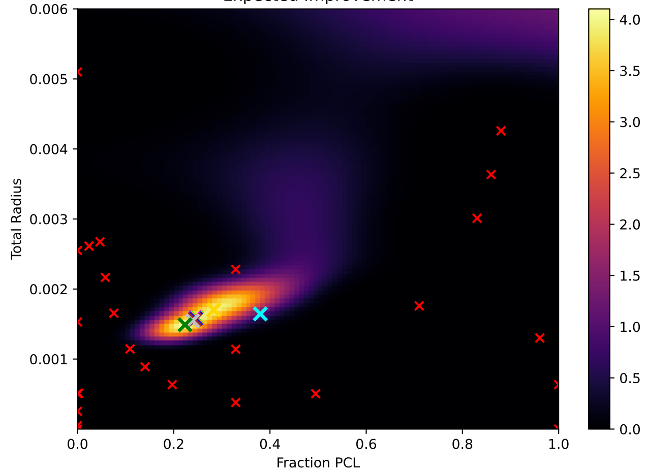
Expected Improvement
