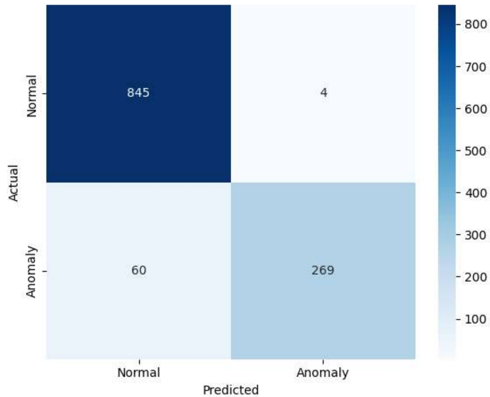
Confusion Matrix - CNN
