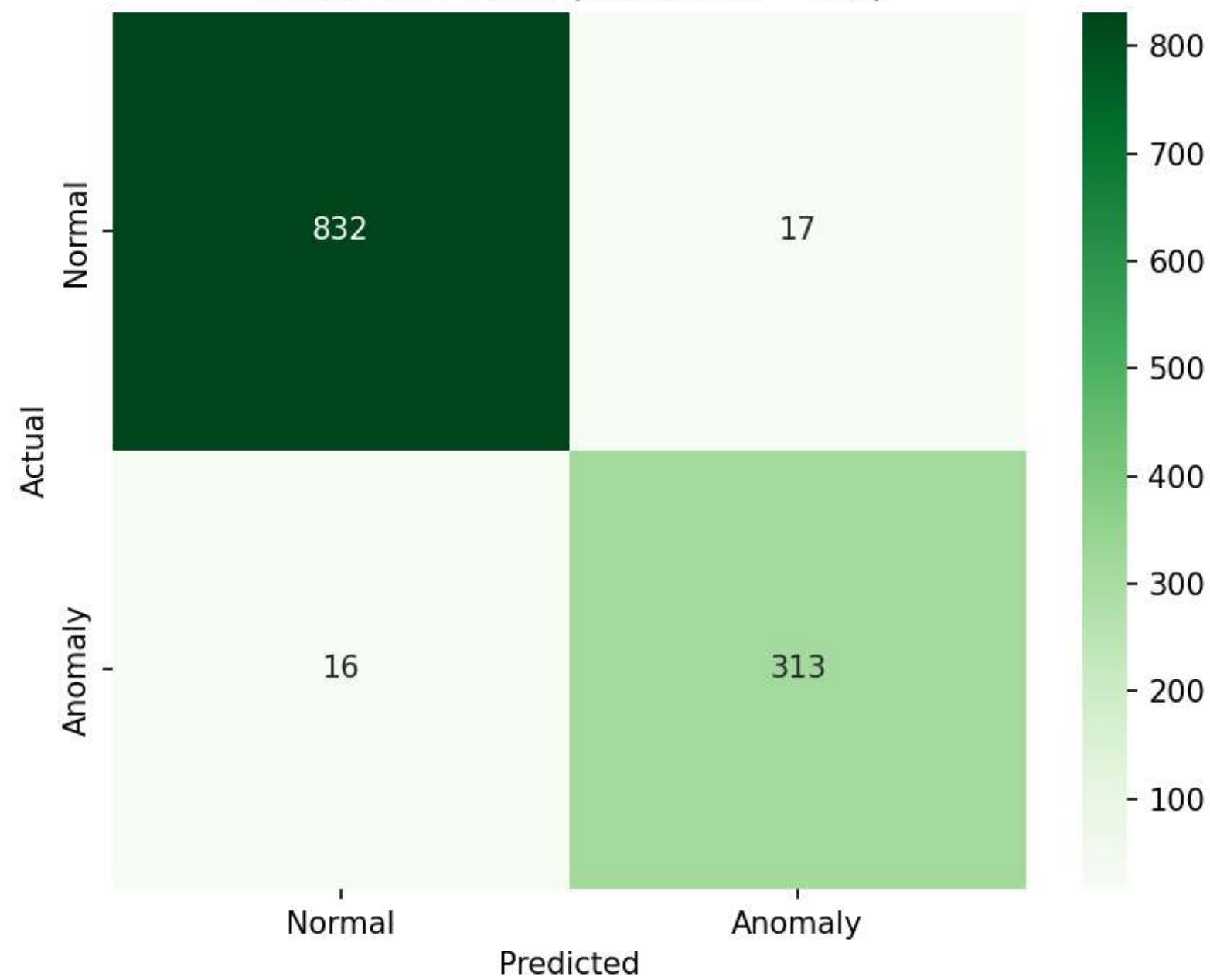
Confusion Matrix (Threshold = 0.2)
