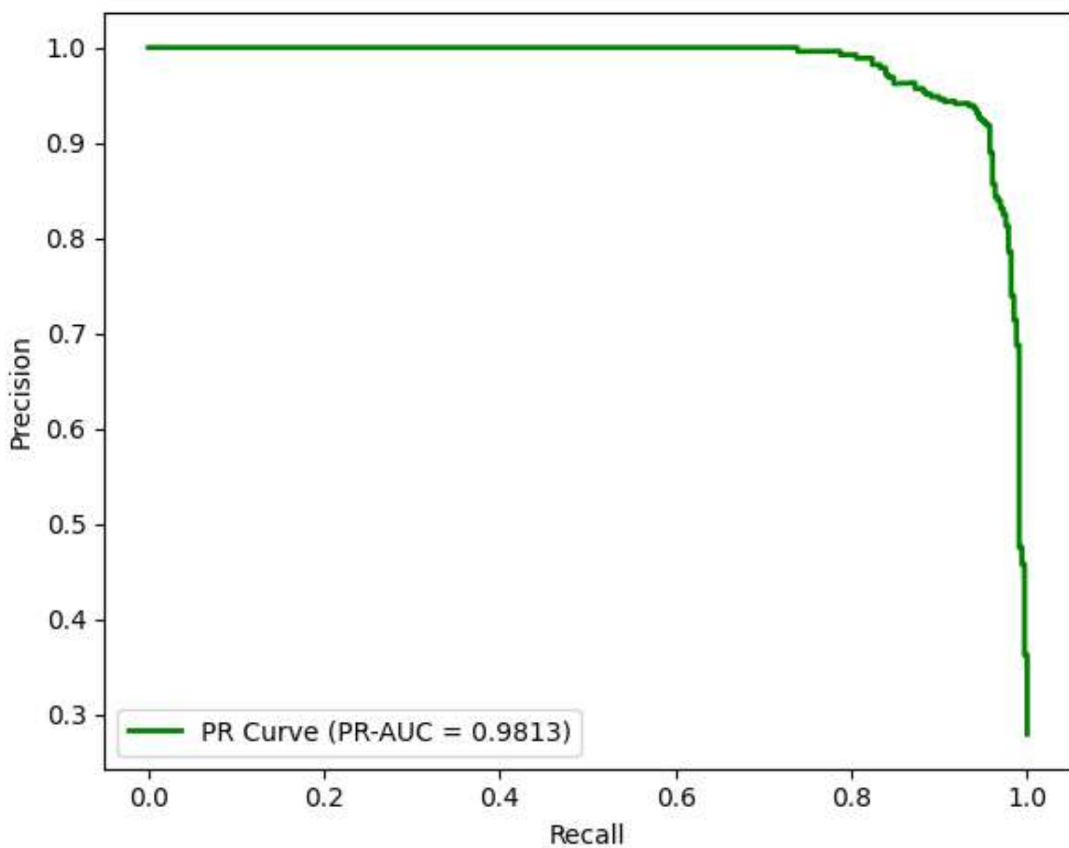
Precision-Recall Curve - CNN
