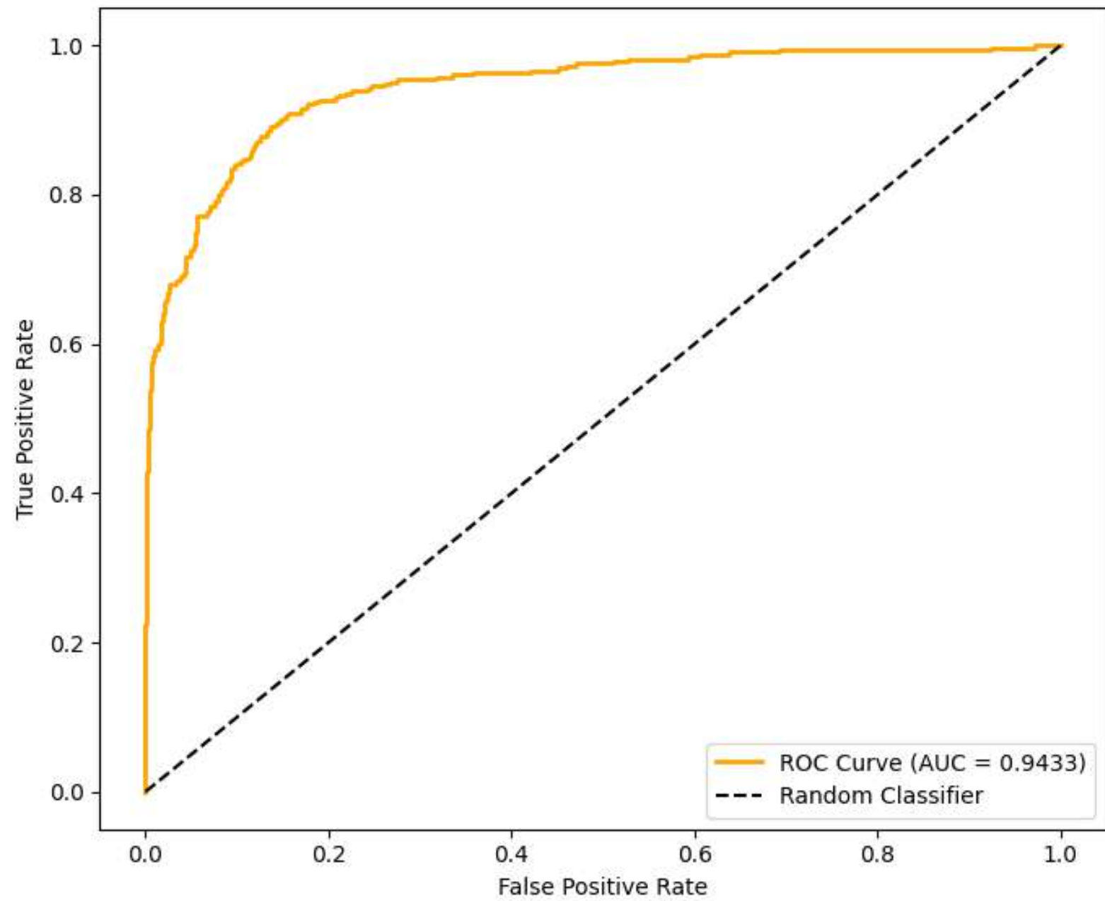
ROC-AUC Curve
