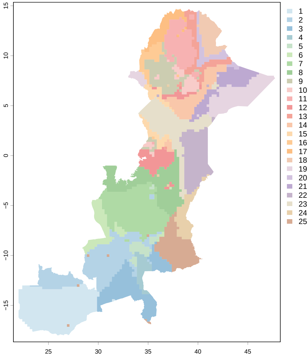
Macrozones for SSA, 25 class model
