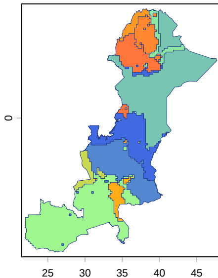
total_precipitation clusters by similar average annual trends
