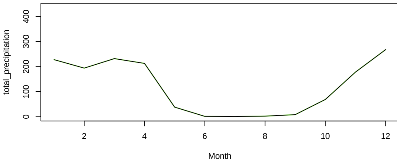
total_precipitation Group 5
