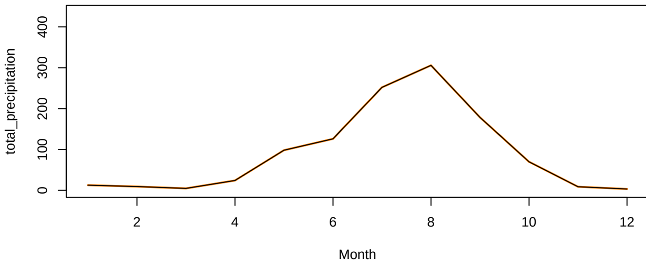
total_precipitation Group 3
