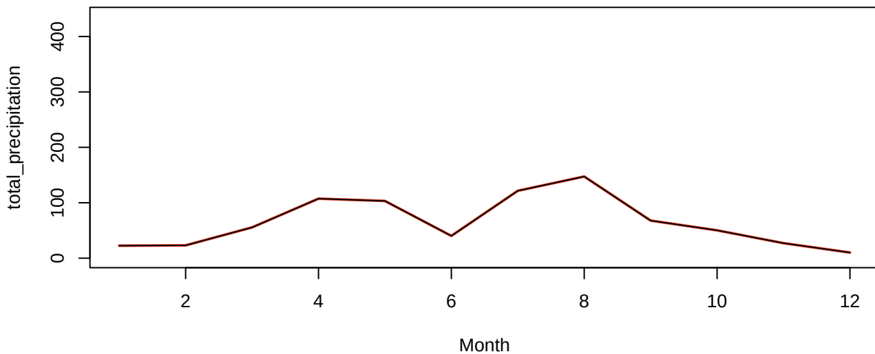
total_precipitation Group 7
