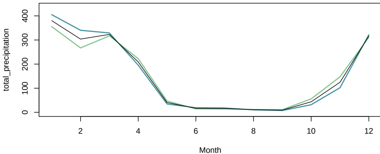
total_precipitation Group 4
