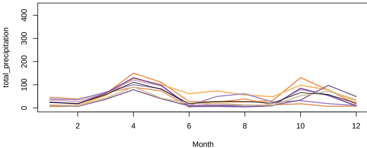
total_precipitation Group 8
