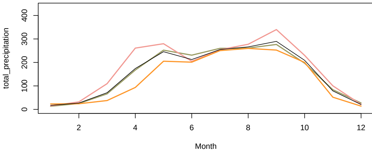
total_precipitation Group 1
