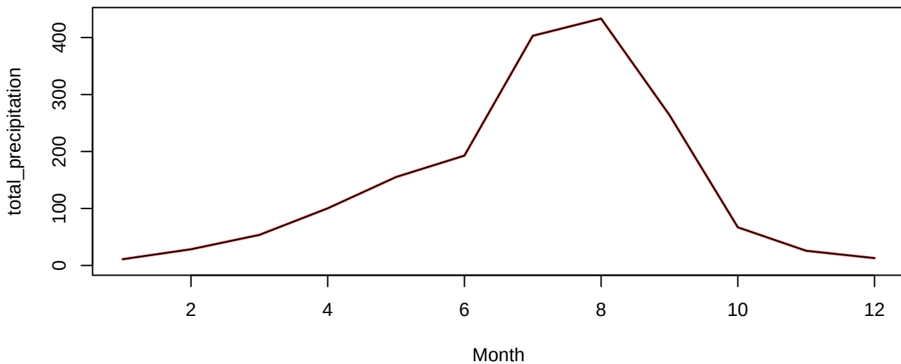
total_precipitation Group 2
