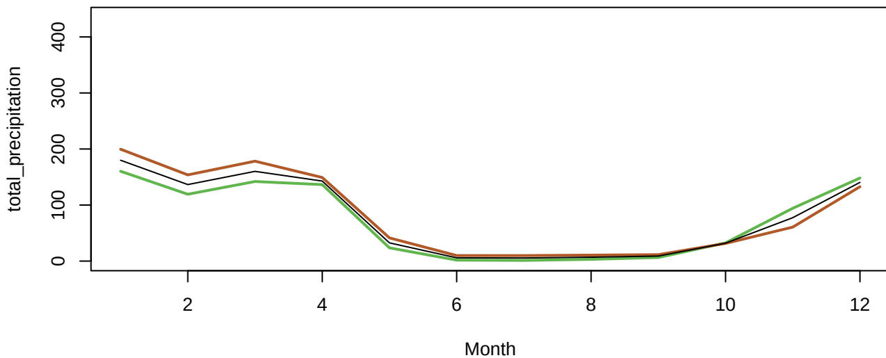
total_precipitation Group 9
