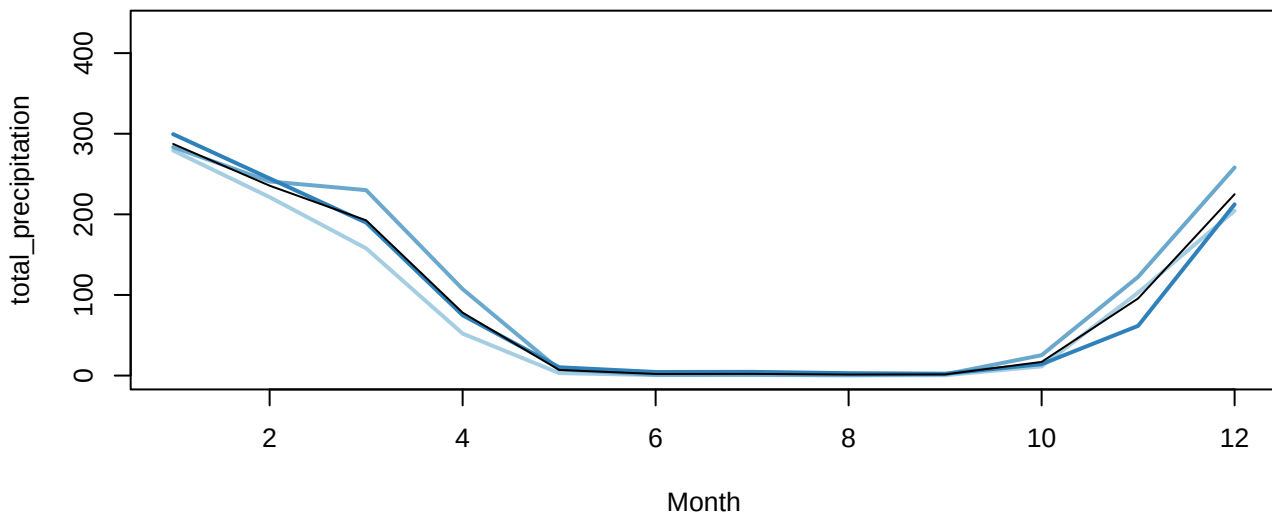
total_precipitation Group 6
