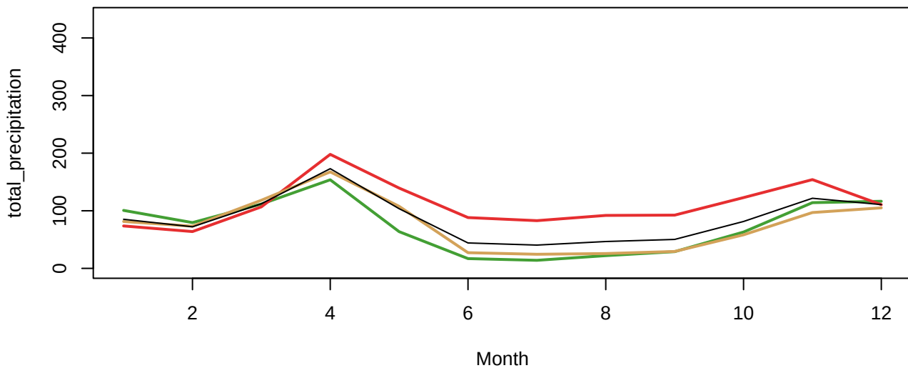
total_precipitation Group 10
