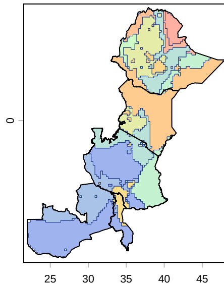
max_temperature clusters by similar average annual trends
