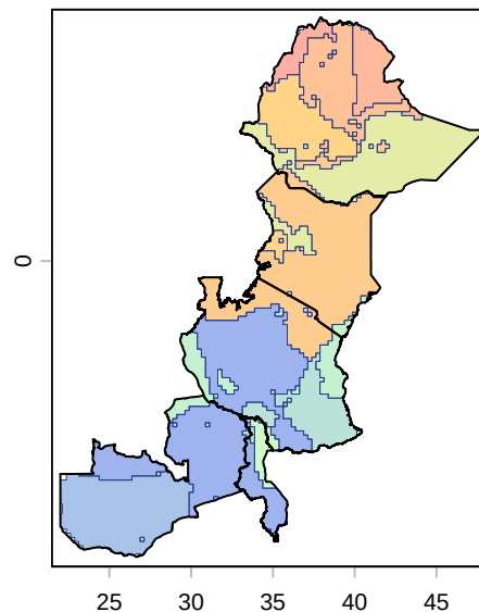
temp_range clusters by similar average annual trends
