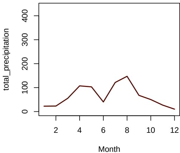
total_precipitation Group 7
