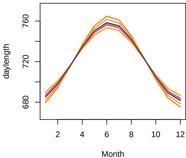
daylength Group 1
