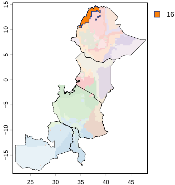
Macrozones with similar total precipitation trends
