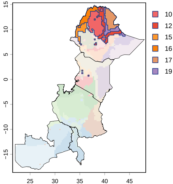
Macrozones with similar daylength trends
