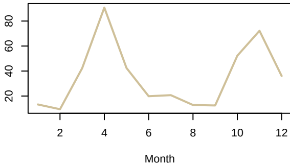
Average Zone Total Precipitation
