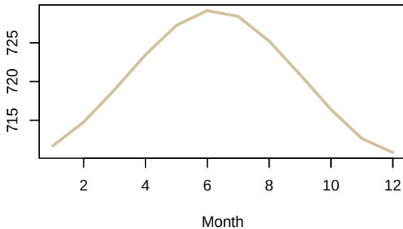
Average Zone Daylength
