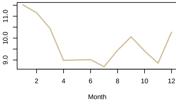
Average Zone Temperature Range
