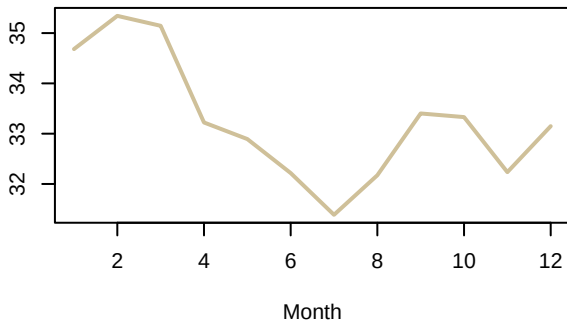
Average Zone Maximum Temperature
