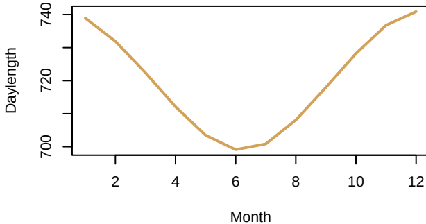
Average Zone Daylength
