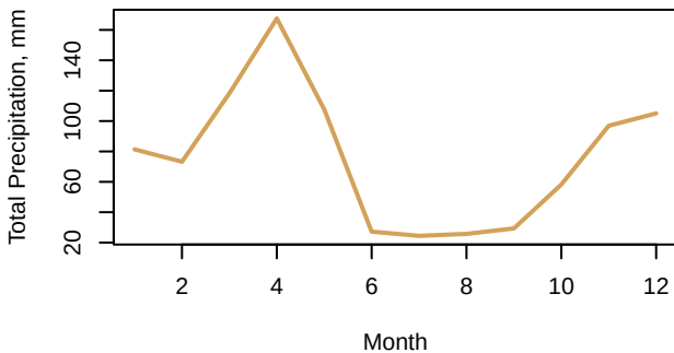
Average Zone Total Precipitation
