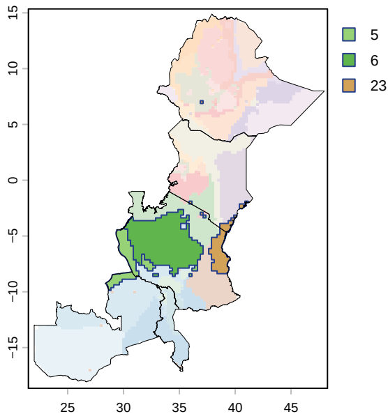
Macrozones with similar daylength trends
