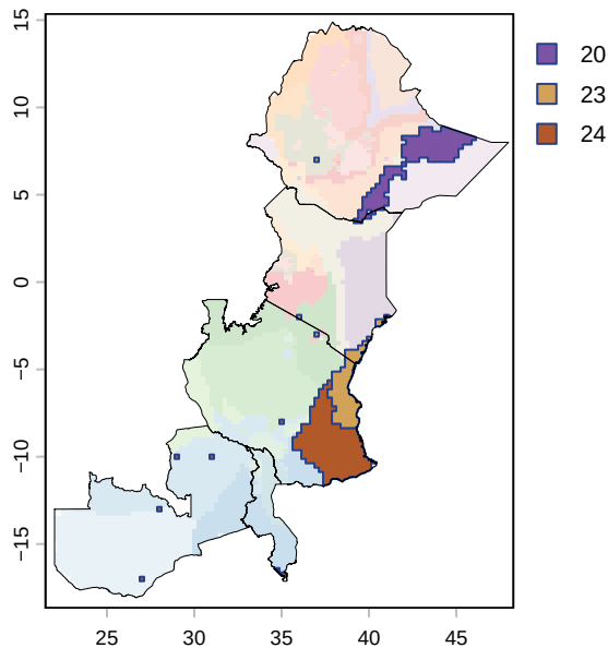
Macrozones with similar maximum temperature trends
