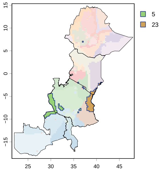
Macrozones with similar temperature range trends
