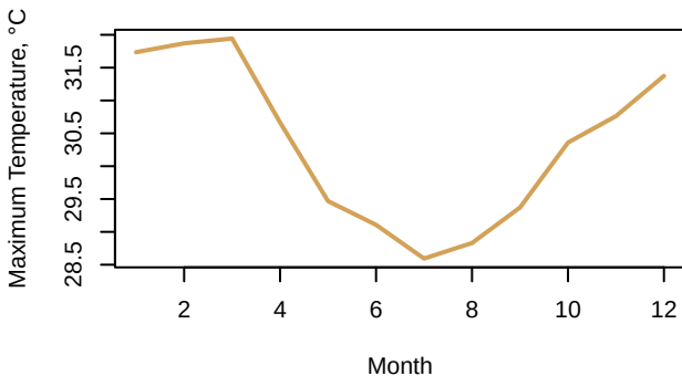
Average Zone Maximum Temperature
