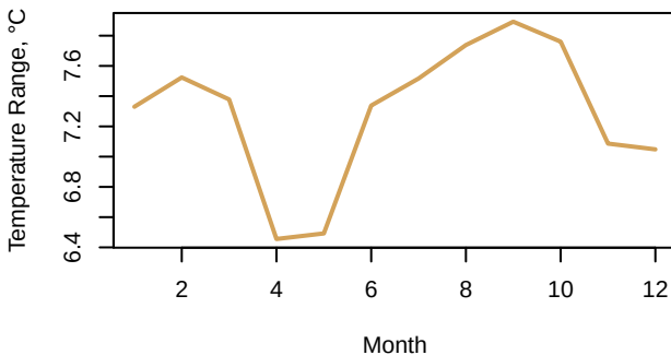
Average Zone Temperature Range
