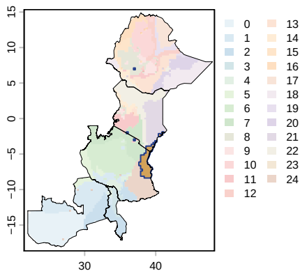
Average Zone Maximum Temperature
