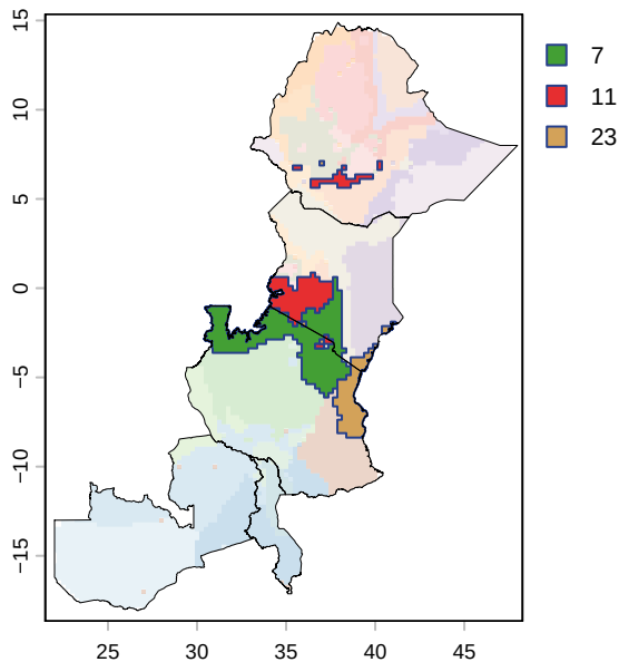
Macrozones with similar total precipitation trends
