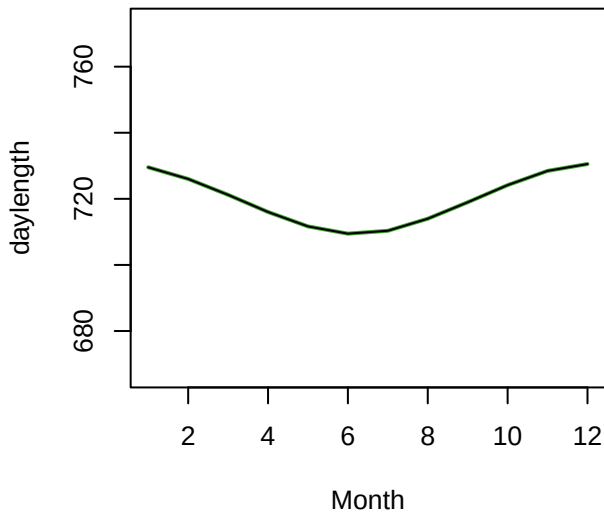
daylength Group 4
