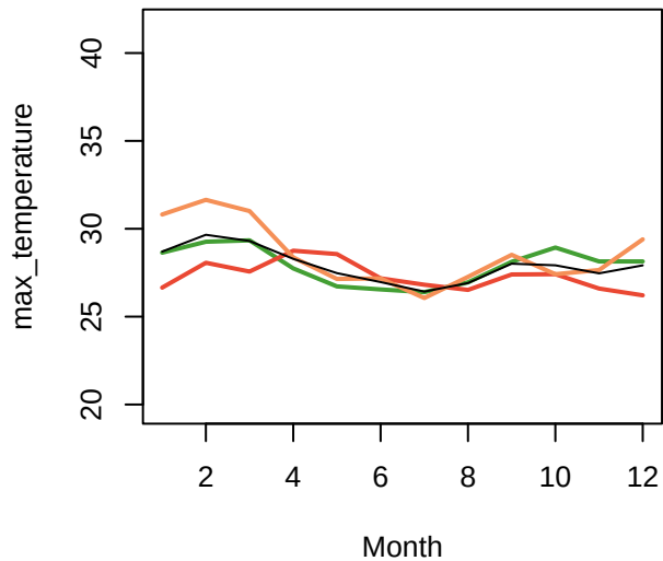
max_temperature Group 10
