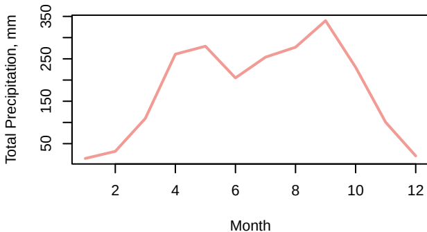
Average Zone Total Precipitation
