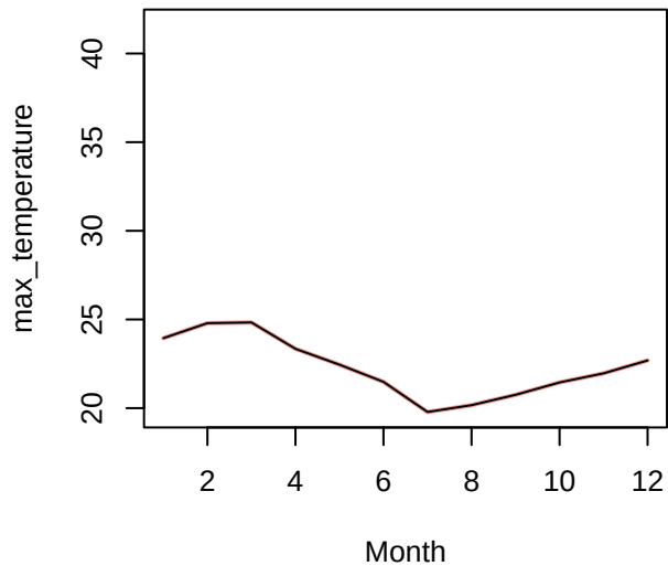
max_temperature Group 5
