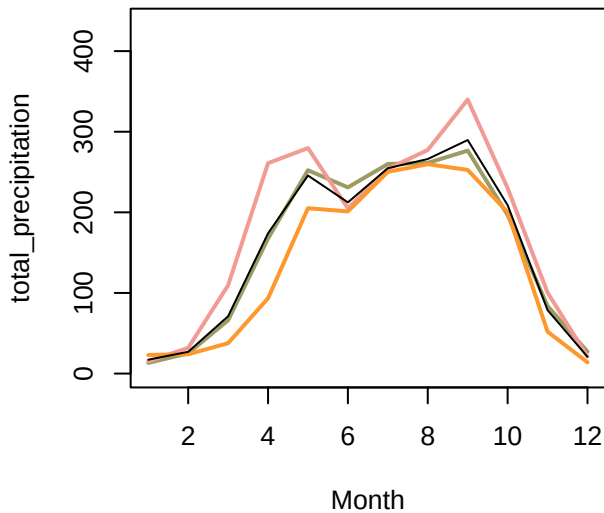
total_precipitation Group 1
