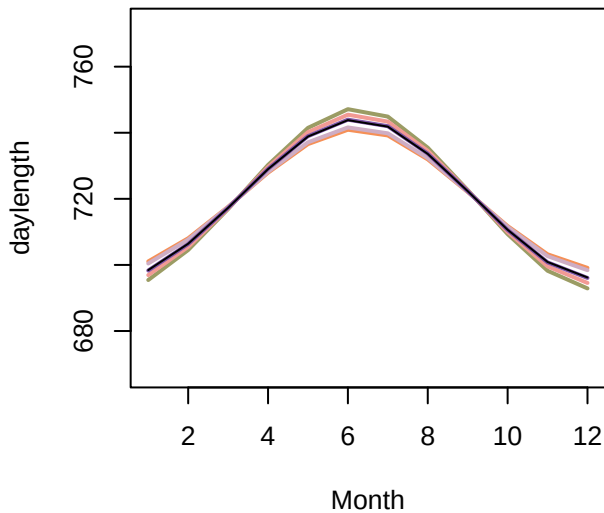
daylength Group 3
