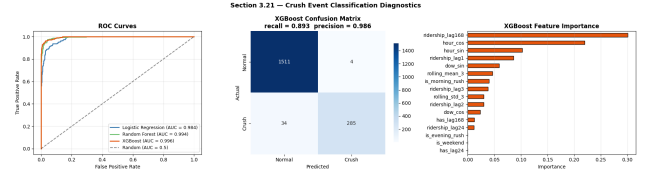
Figure 6: The crush event classification diagnostics. On left: ROC curves for all three models (AUC 0.984 to 0.996). At center: XGBoost confusion matrix (4 false positives and 34 false negatives). On right: XGBoost feature importance, weekly lag dominates.
