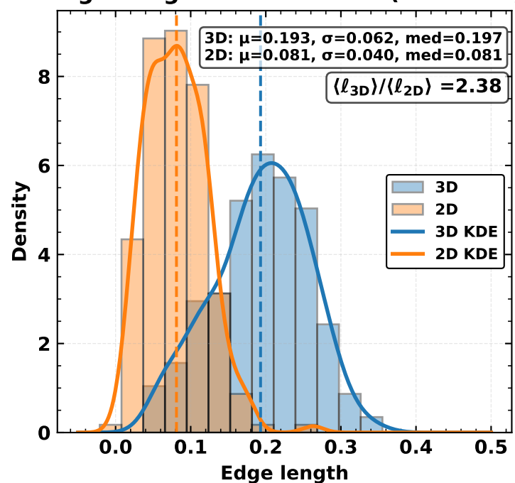
Edge Length Distributions (3D vs 2D)
