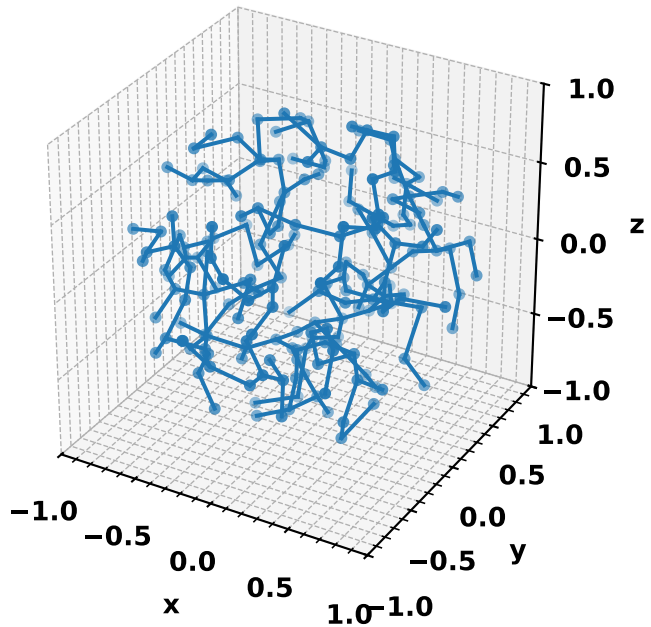
3D MST (N=200, Uniform)
