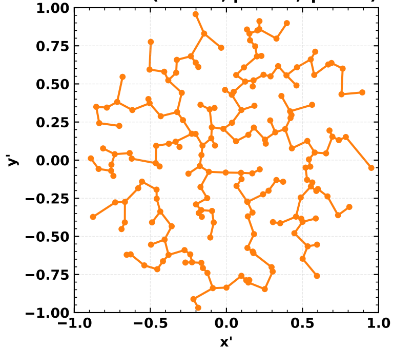
2D MST ( \alpha=0.0^\circ , \beta=0.0^\circ , \gamma=0.0^\circ )
