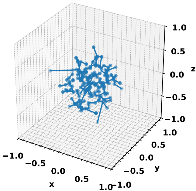
3D NN (N=200, Gaussian, \sigma=0.25 )
