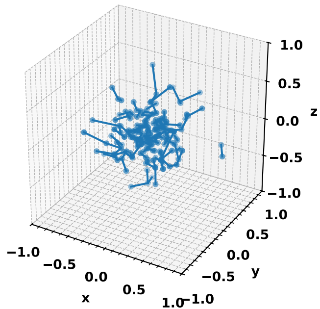
3D NN (N=200, Plummer, a=0.25)
