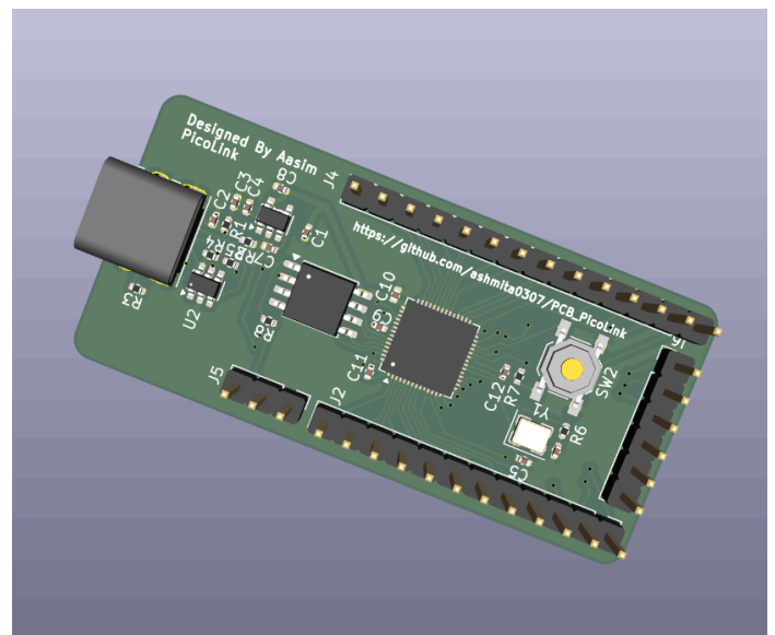
Figure 6.2 RP2040 PCB-(b)
