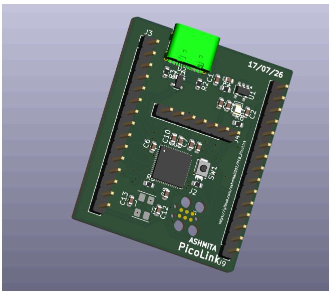
Figure 6.1 PCB Design-(a)
