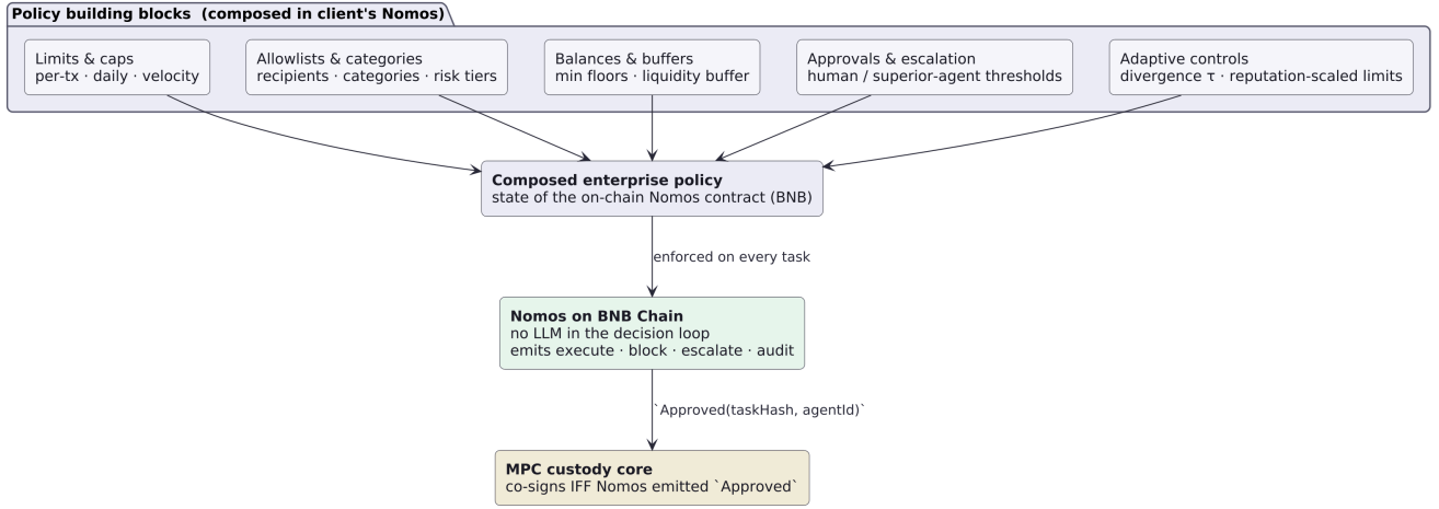
Figure 5: Composable policy. An enterprise assembles building blocks into a policy stored as state in its own Nomos contract on BNB Chain. The on-chain engine enforces it on every task and emits the verdict; the MPC custody core co-signs only on Approved.
